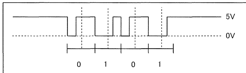
ELECTRICAL OUTPUT OF DIAGNOSIS INFORMATION
