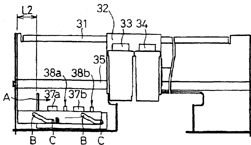
FIG. 11 PRIOR ART
