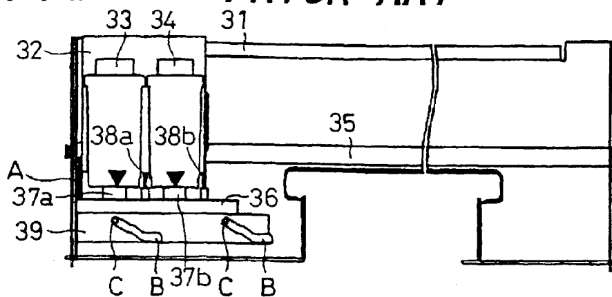
FIG. 9 PRIOR ART
