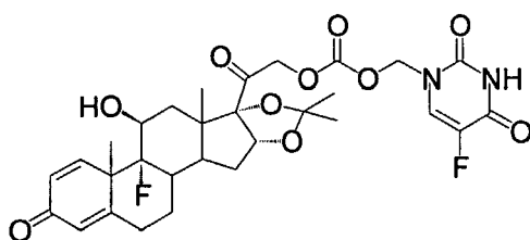
TC-32 (codrug of triamcinolone acetonide with 5-FU via formaldehyde linkage)
