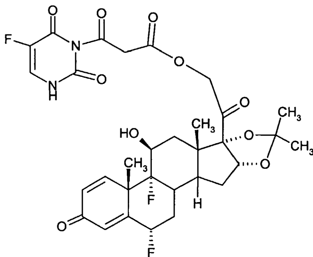
5FU-fluocinolone acetonide (via oxalate linker).
