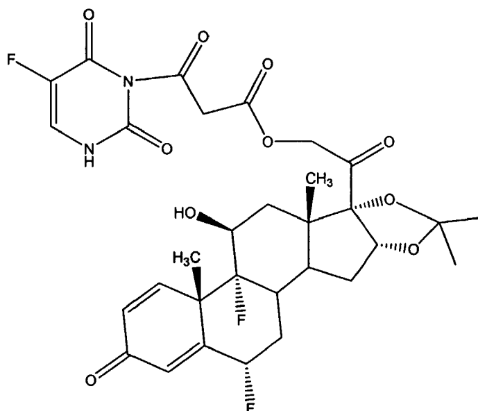
5FU-flucinolone acetonide (III),
