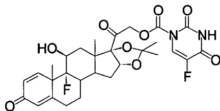
G-427.1 (direct codrug of triamcinolone acetonide with 5-FU)
