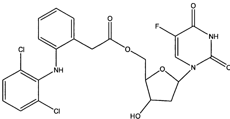
Co-drug of Floxuridine with Diclofenac (1:1)
