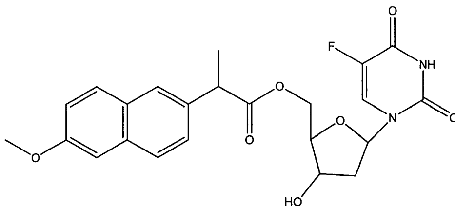
Co-drug of Floxuridine with Naproxen (1:1)
