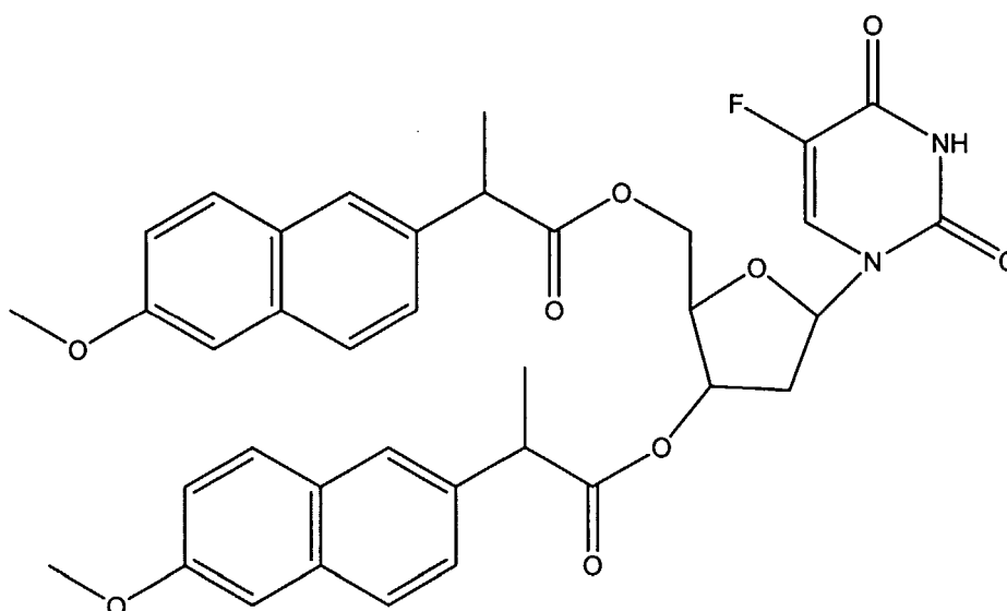
Co-drug of Floxuridine with Naproxen (1:2)
