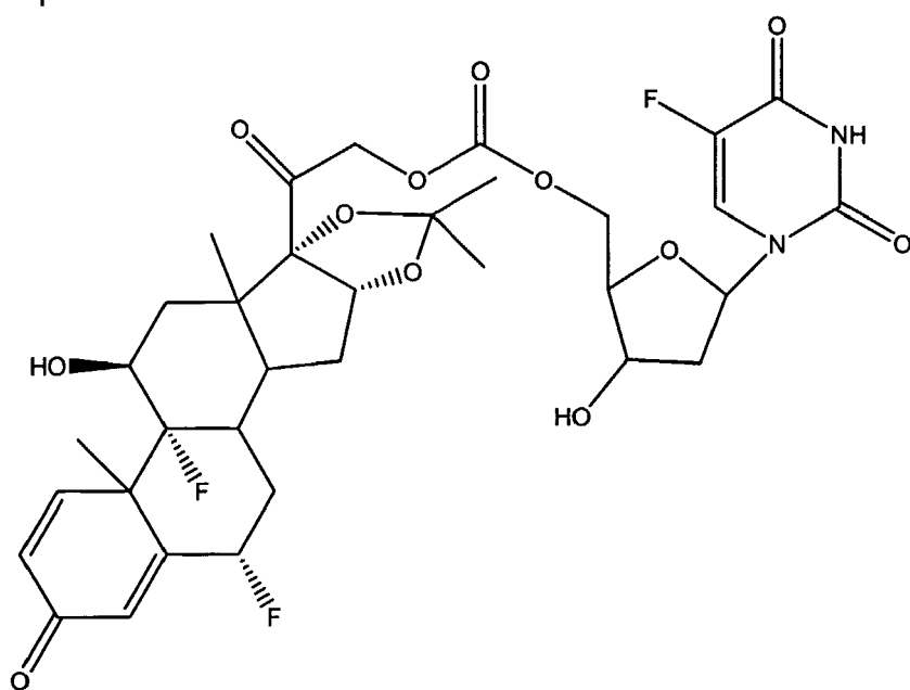
Co-drug of Floxuridine with Fluocinolone acetonide (1:1)
