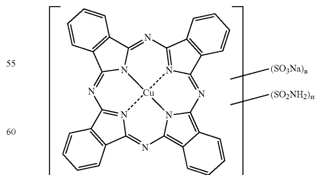
Blue dye-1
