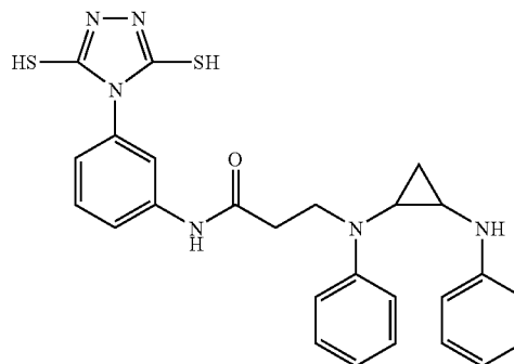
Base precursor-1
