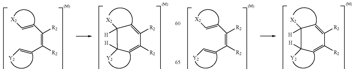
Reaction formula (1)
