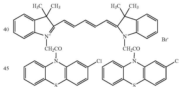
Cyanine dye-1
