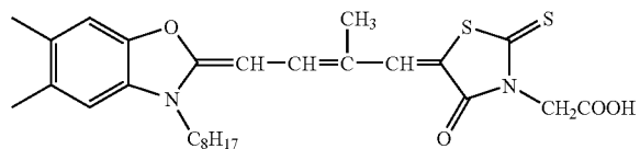
Spectral sensitizing dye A
