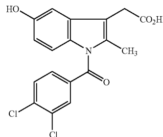
[0044] [1-(3,4-dichlorobenzoyl)-5-hydroxy-2-methyl-1H-indol-3-yl]acetic acid
