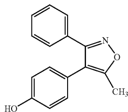
4-(5-methyl-3-phenylisoxazol-4-yl)phenol
