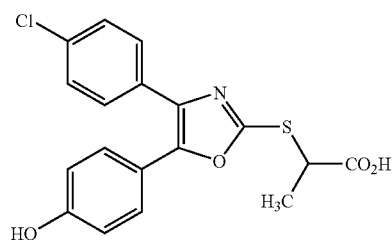
[0296] 2-[[4-(4-chlorophenyl)-5-(4-hydroxyphenyl)-1,3-oxazol-2-yl]thio]propionic acid
