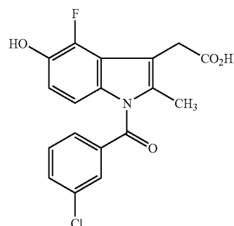
[0041] [1-(3-chlorobenzoyl)-6-fluoro-5-hydroxy-2-methyl-1H-indol-3-yl]acetic acid
