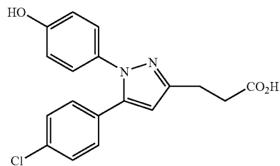
[0297] 3-[5-(4-chlorophenyl)-1-(4-hydroxyphenyl)-1H-pyrazol-3-yl]propionic acid
