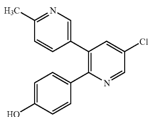
4-(5-chloro-6'-methyl-3,3'-bipyridin-2-yl)phenol
