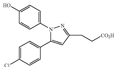
3-[5-(4-chlorophenyl)-1-(4-hydroxyphenyl)-1H-pyrazol-3-yl]propionic acid
