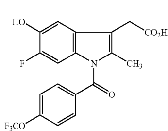
[0087] 2-[1-(4-trifluoromethoxybenzyl)-5-hydroxy-2-methyl-1H-indol-3-yl]propionic acid
