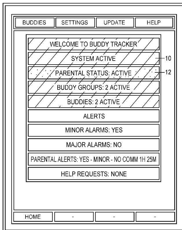
OPENING SCREEN
