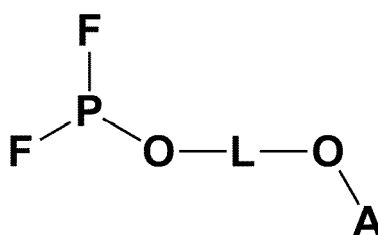
[Chemical Formula 1]
