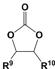
[Chemical Formula 3]
