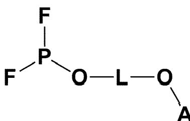
[Chemical Formula 1]
