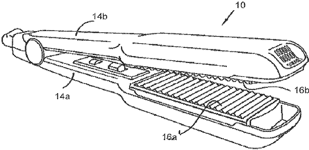
Figure 2 (prior art)
