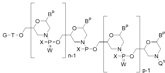
[C-1-1]
