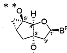
[4c1]
