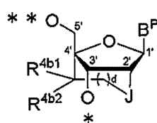
[4b1]
