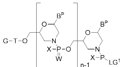
[A-1-3]
