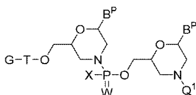
[C-0]
