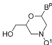
[B-0]
