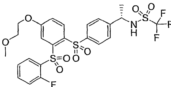
Compound XXXXV
