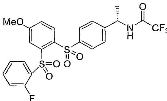
Compound 17
