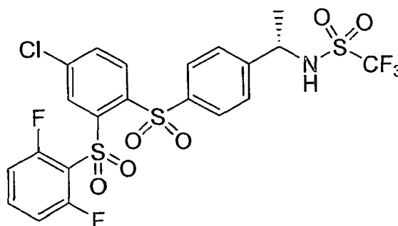
Compound VII
