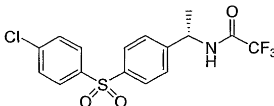
Compound 5
