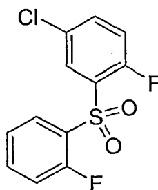
Compound 41
