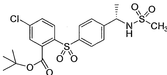
Compound 25
