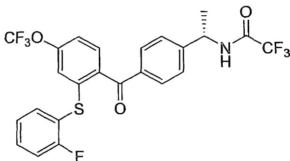
Compound 35
