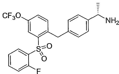
Compound 33
