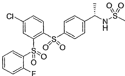
Compound IV
