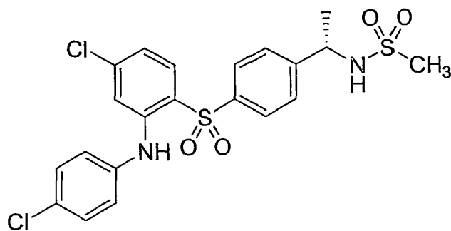
Compound XVII
