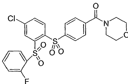
Compound XXVIII
