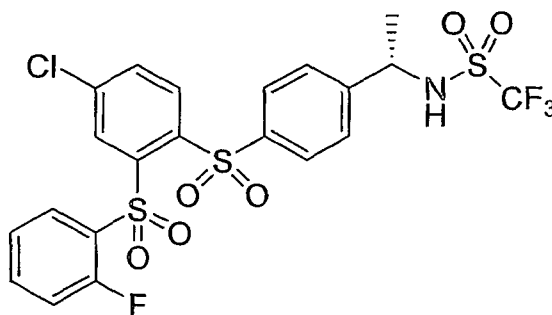
Compound V
