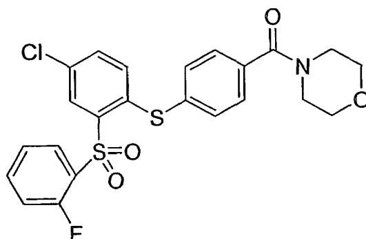
Compound XXVII
