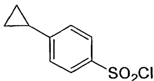
Compound 45
