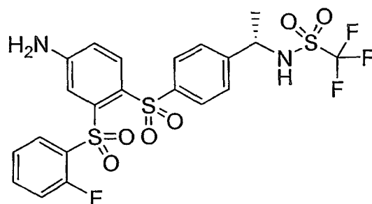
Compound XXXIII
