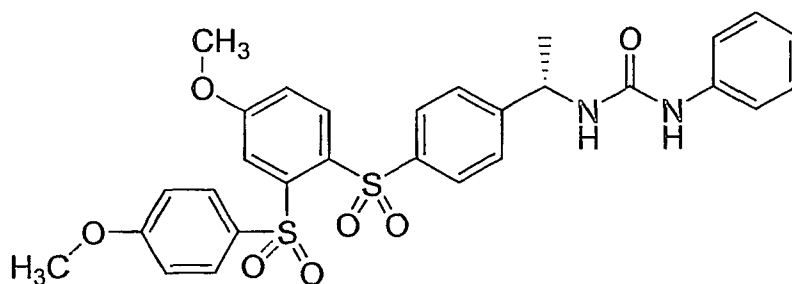
Compound III
