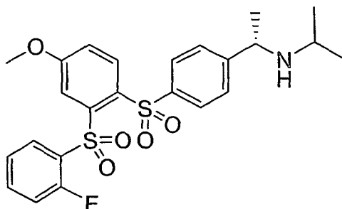
Compound XXXXXI.
