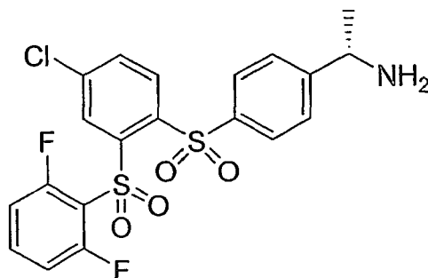
Compound 9
