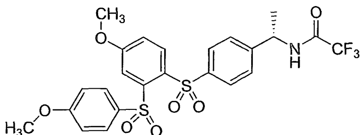
Compound 3
