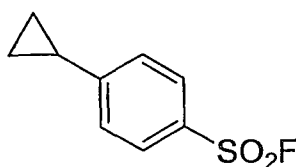
Compound 46
