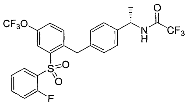
Compound 32
