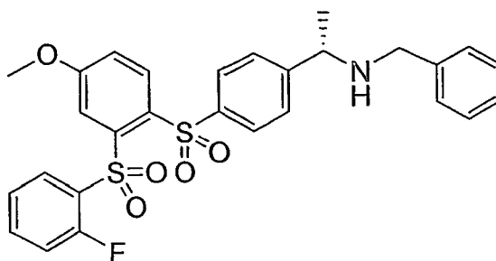
Compound XXXXXIII
