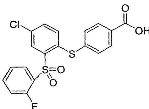
Compound 42
