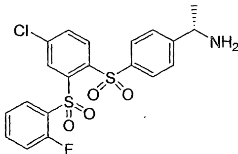
Compound 7
