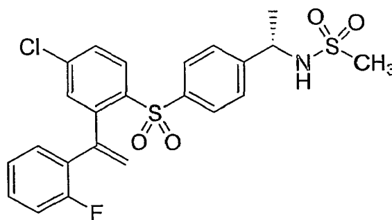
Compound XV
