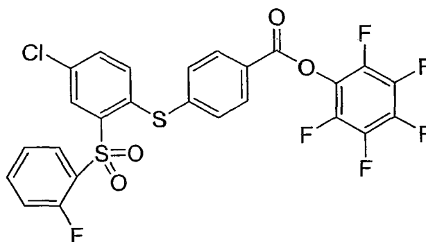
Compound 43
