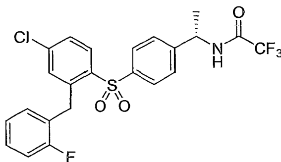
Compound 22
