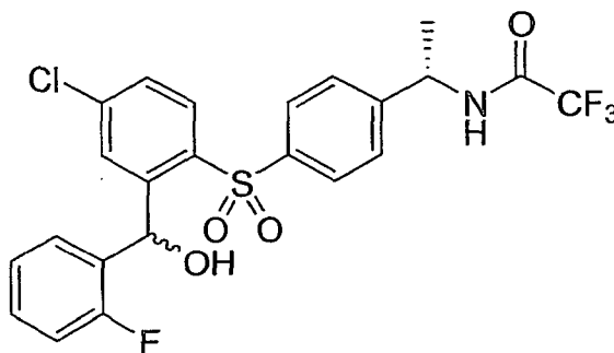
Compound 21
