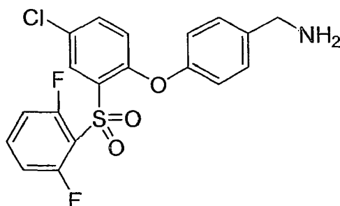
Compound 15
