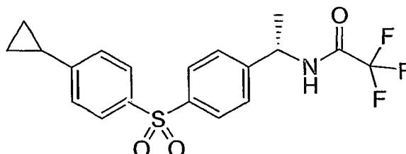
Compound 47
