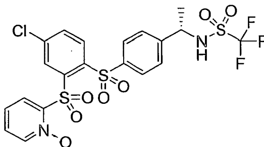
Compound XXXVI
