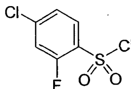
Compound 53
