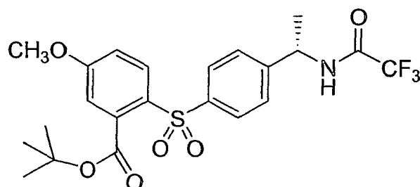
Compound 20
