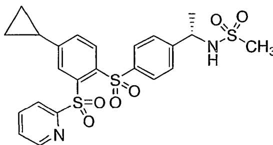
Compound XXXXXVI
