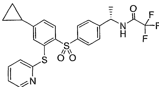
Compound 48
