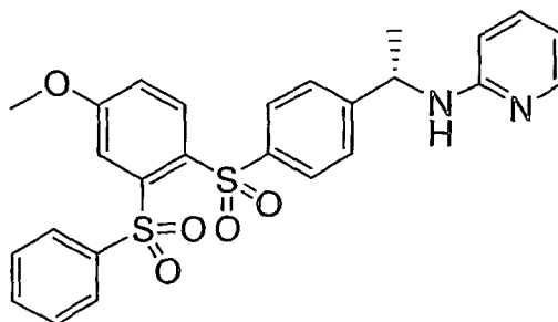
Compound XXXXXIV
