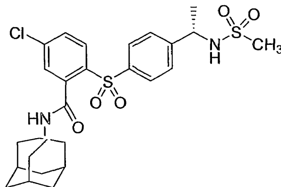
Compound XVI
