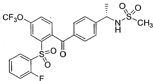
Compound 37
