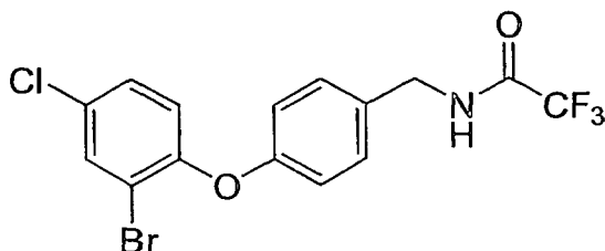
Compound 13
