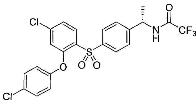
Compound 28
