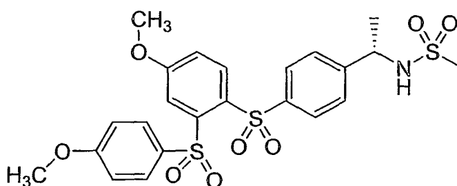
Compound I
