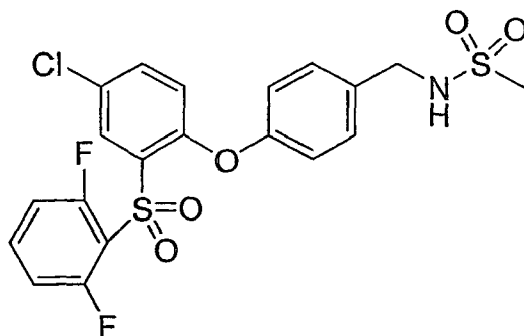
Compound IX
