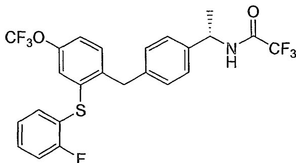
Compound 31
