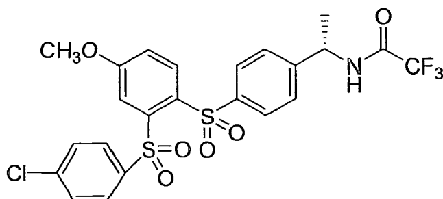
Compound 39
