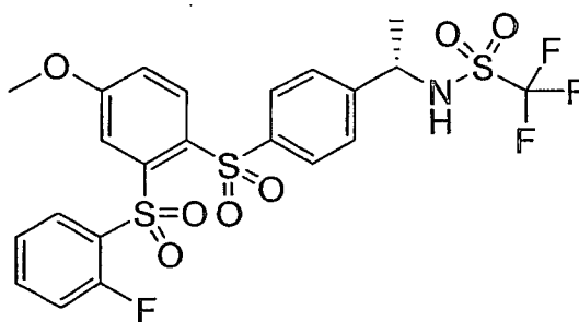
Compound XXXIX
