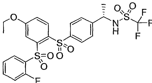
Compound XXXXIV
