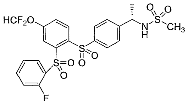
Compound XI
