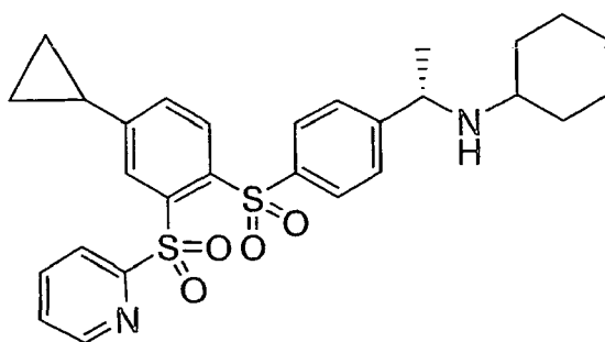
Compound XXXXVIII
