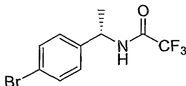
Compound 1
