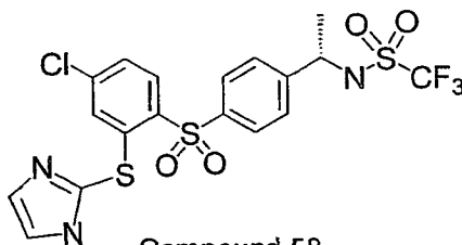
Compound 58
