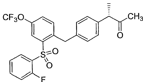
Compound XXI
