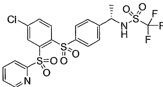
Compound XXXV
