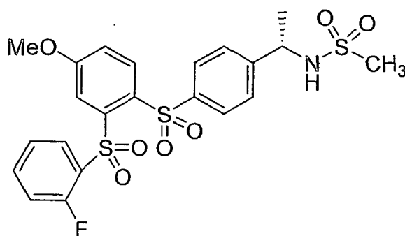
Compound 16
