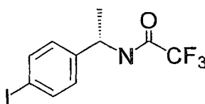
Compound 55
