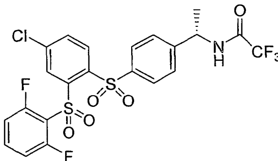
Compound 8
