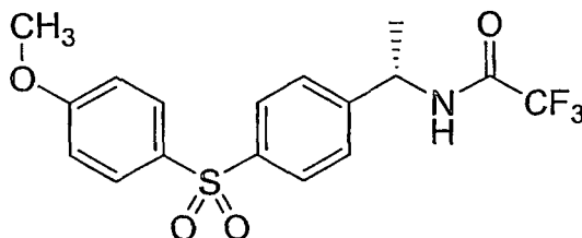
Compound 2
