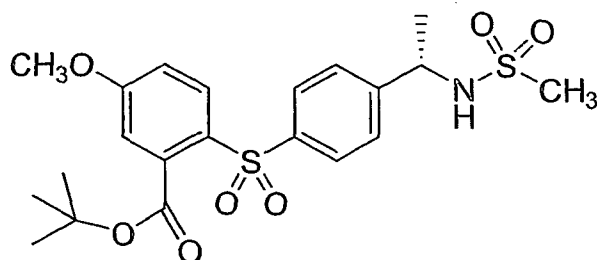
Compound XII
