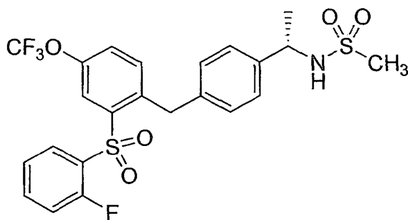
Compound 34
