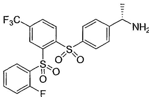
Compound 11
