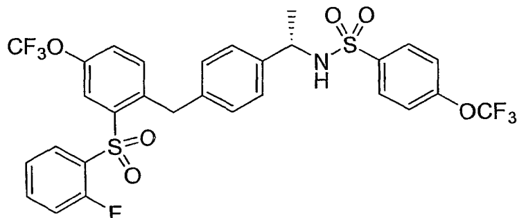
Compound XX
