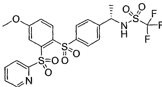
Compound XXXXXV
