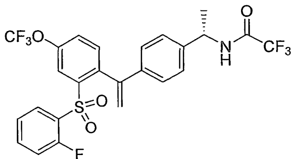
Compound 38
