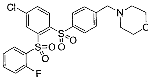
Compound XXXXX
