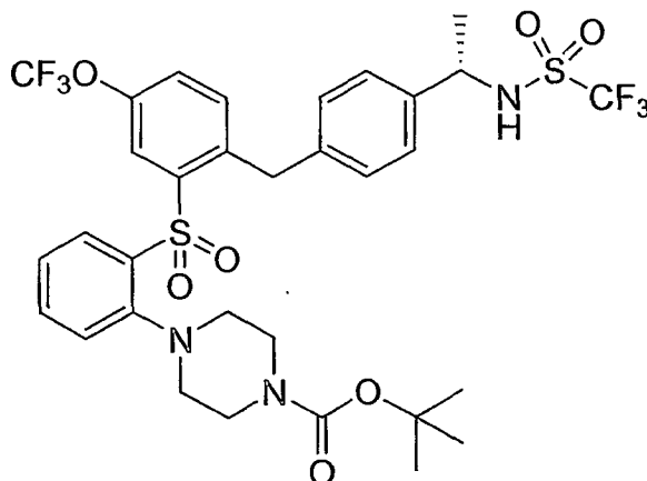
Compound XXIII
