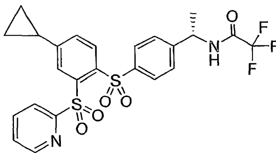
Compound 49
