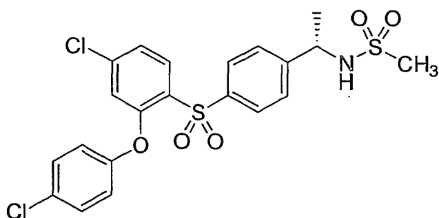
Compound XVIII
