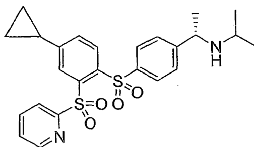
Compound XXXXVI
