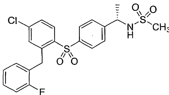
Compound XIII
