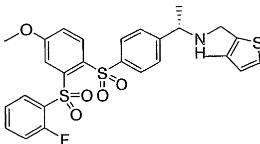
Compound XXXXXII
