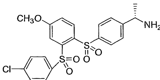
Compound 40
