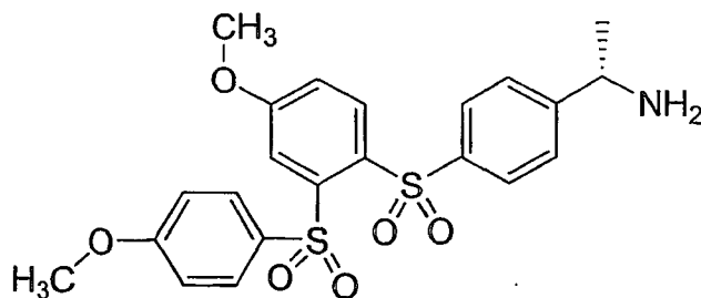
Compound 4
