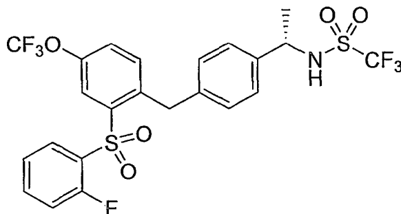
Compound XIX
