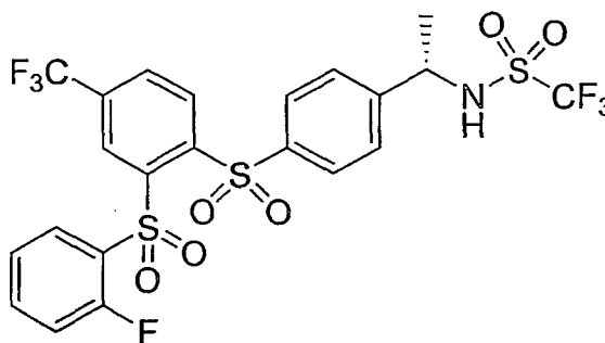
Compound VIII
