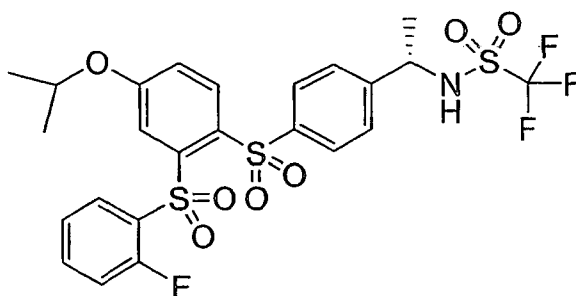
Compound XXXXII
