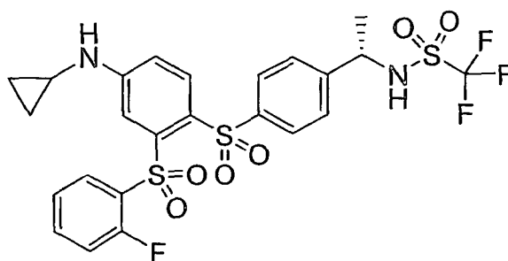
Compound XXXIV
