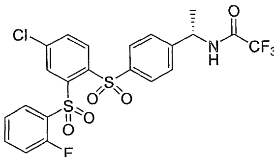
Compound 6
