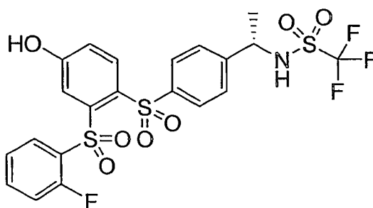
Compound XXXXI
