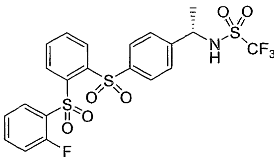
Compound VI
