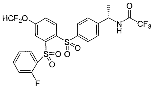
Compound 19
