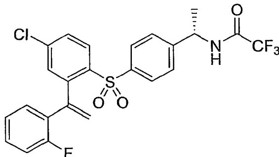
Compound 24
