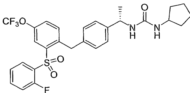
Compound XXII
