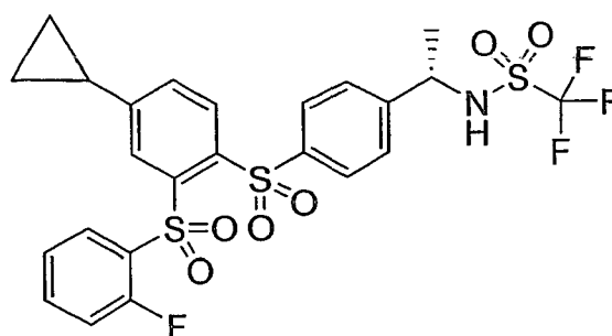
Compound XXX
