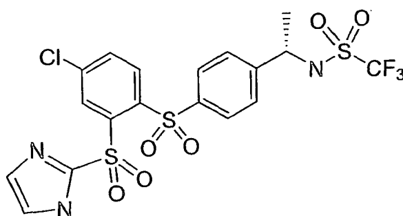
Compound XXXXXVII
