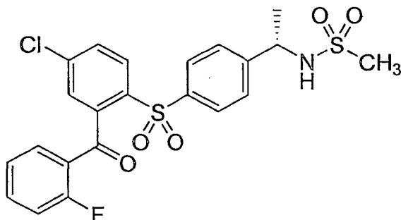
Compound XIV
