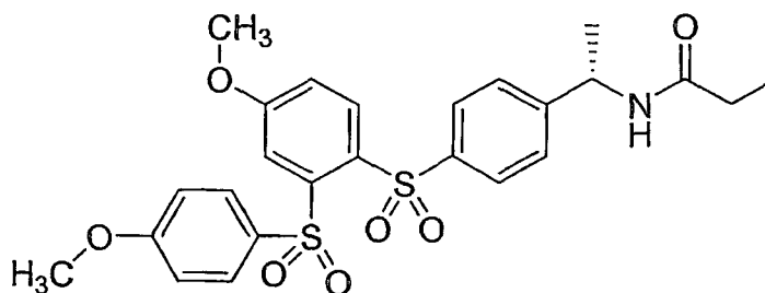
Compound II
