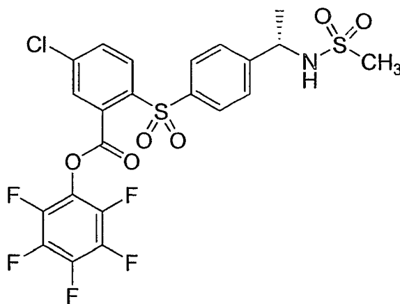
Compound 26
