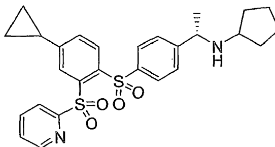
Compound XXXXVII
