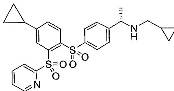
Compound XXXXIX
