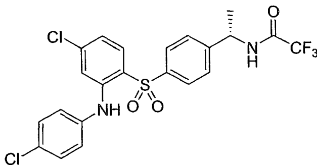
Compound 27
