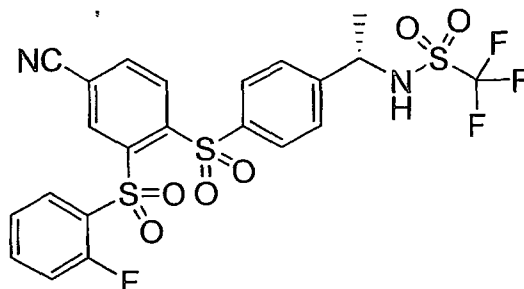
Compound XXXII
