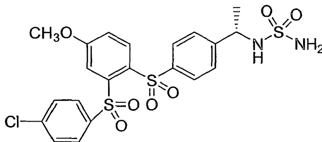
Compound XXVI
