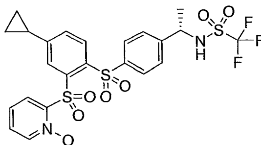
Compound XXXI
