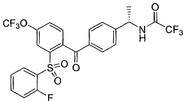
Compound 36
