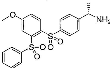
Compound 52
