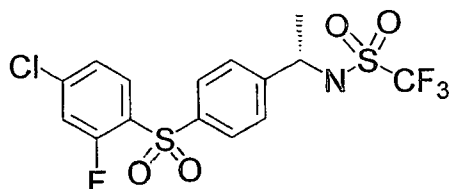
Compound 57
