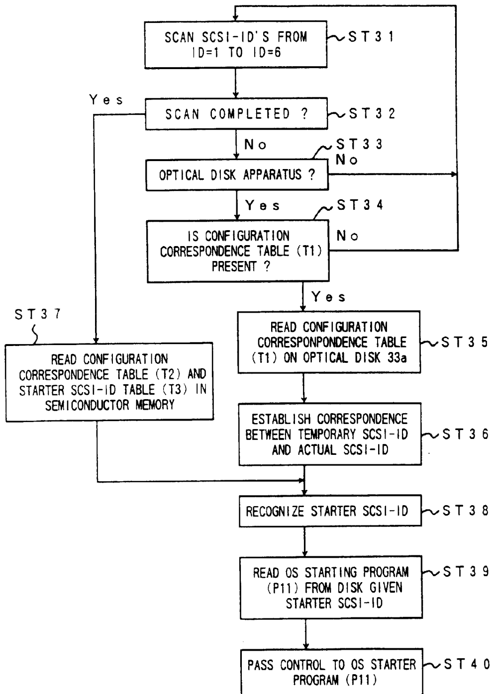
FLOW CHART OF OPERATIONS OF BOOT PROGRAM
