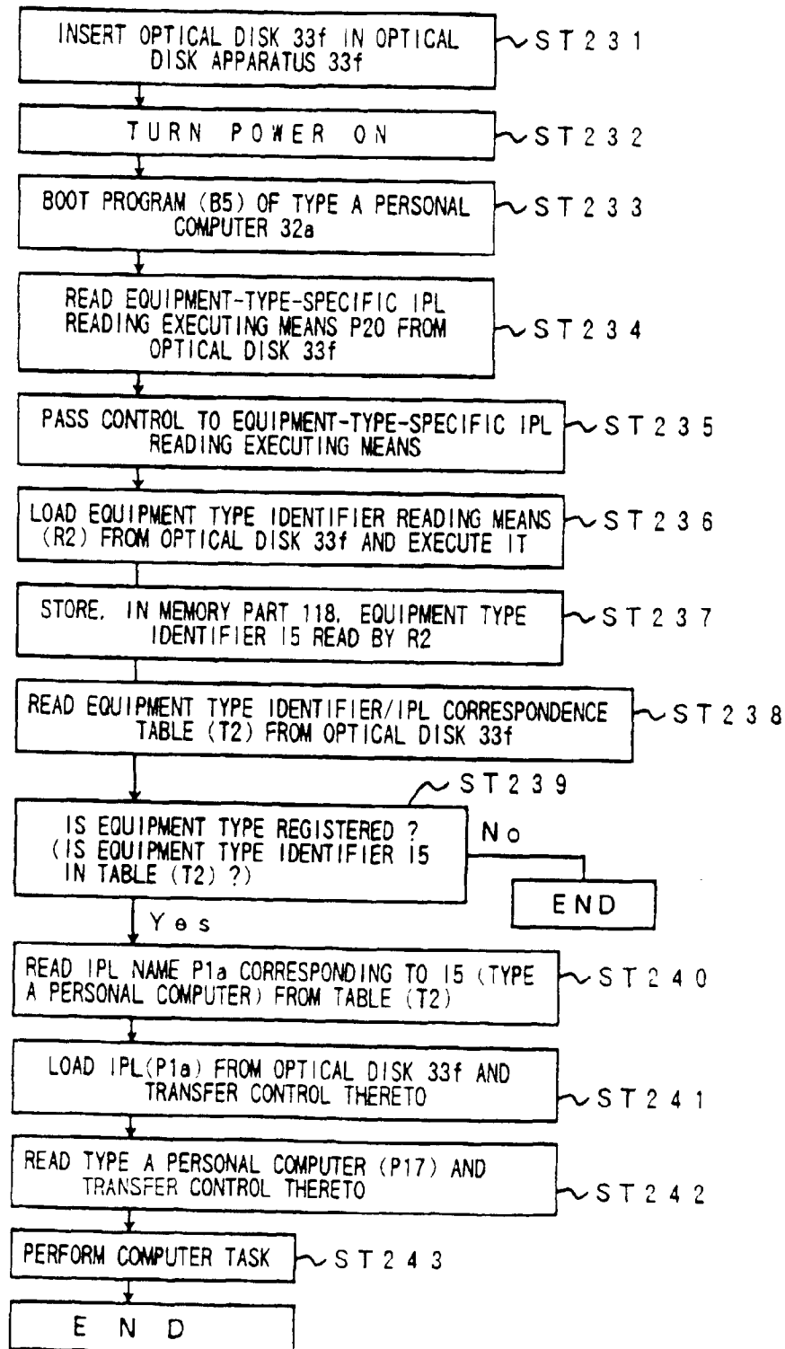
FLOW CHART OF OPERATIONS OF FIG. 38
