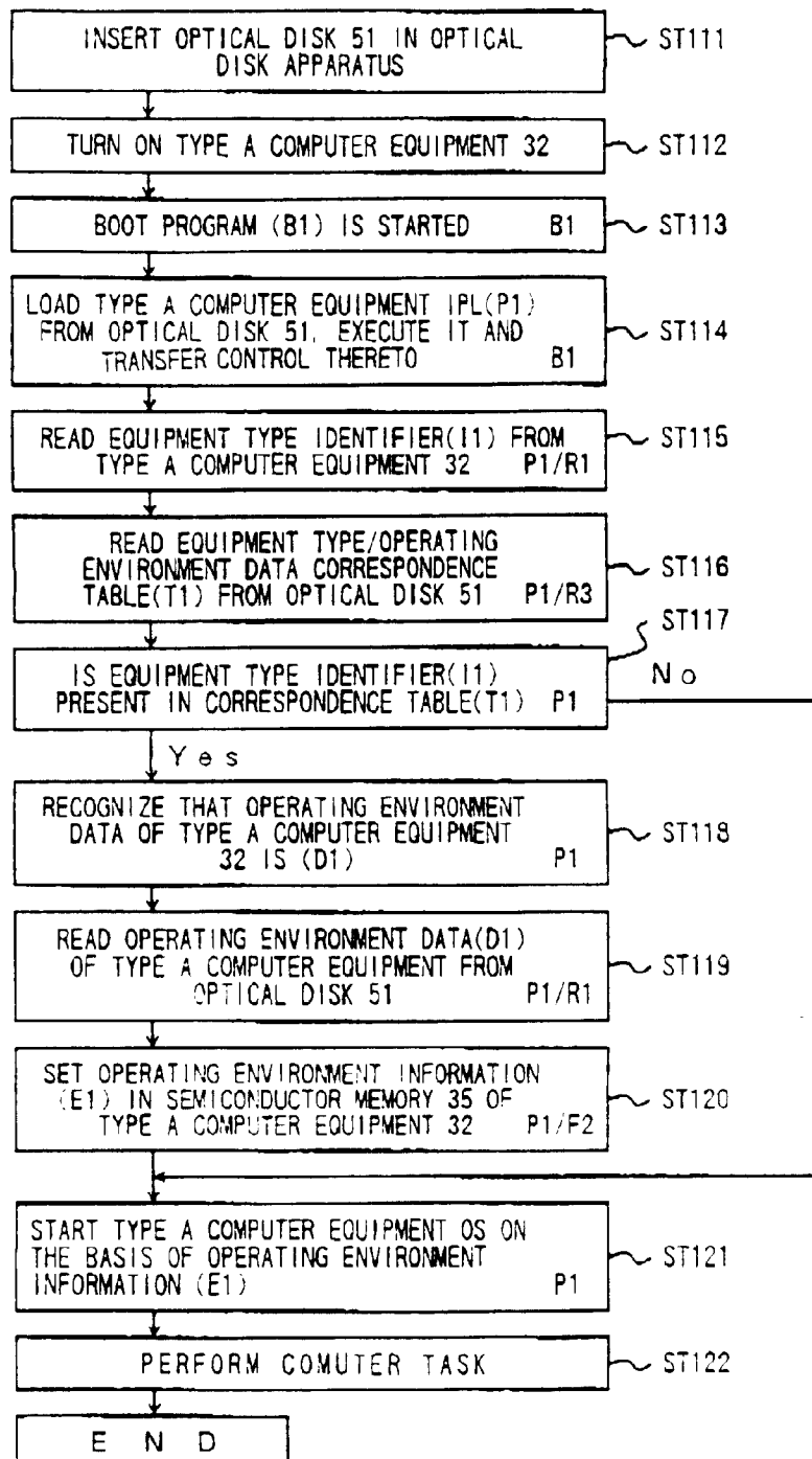
FLOW CHART OF ENVIRONMENTAL INFORMATION REWRITING OF FIG. 13
