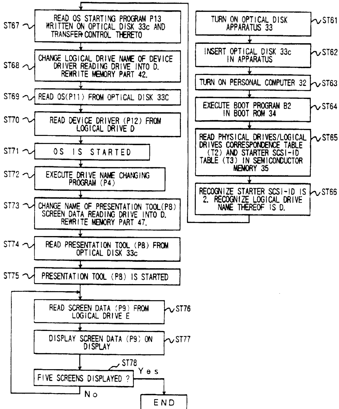
FLOW CHART OF PRESENTATION TOOL OF FIG. 6
