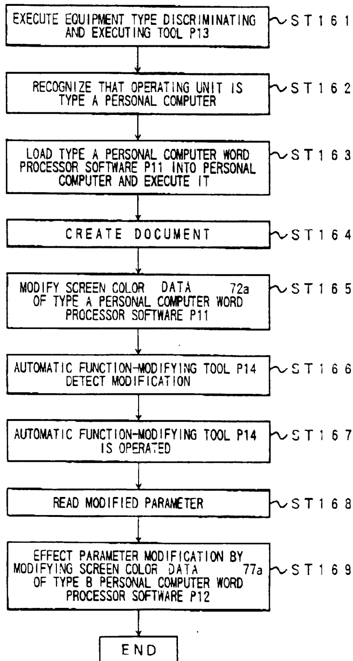
FLOW CHART OF OPERATIONS OF SECOND APPLICATION OF THIRD EMBODIMENT
