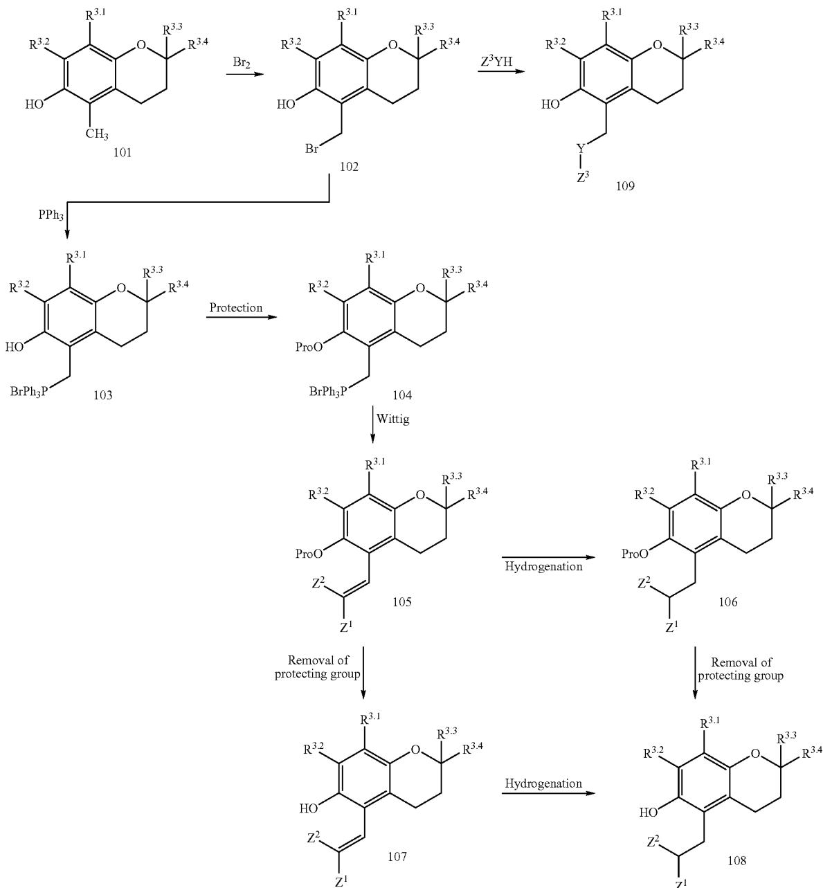
Reaction Scheme 1
