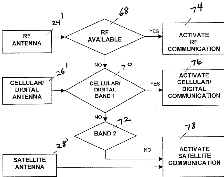
Fig. 6 Data Processing of the Communication Module
