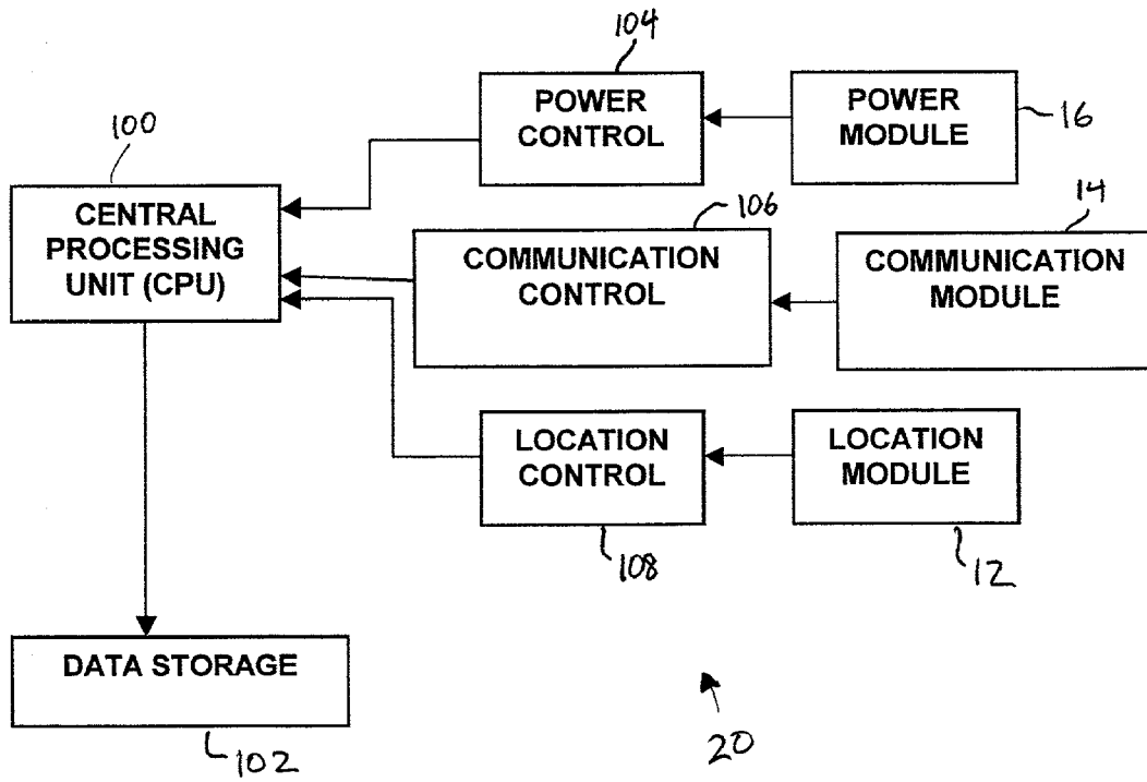
Fig. 10 The Processor Module (E)
