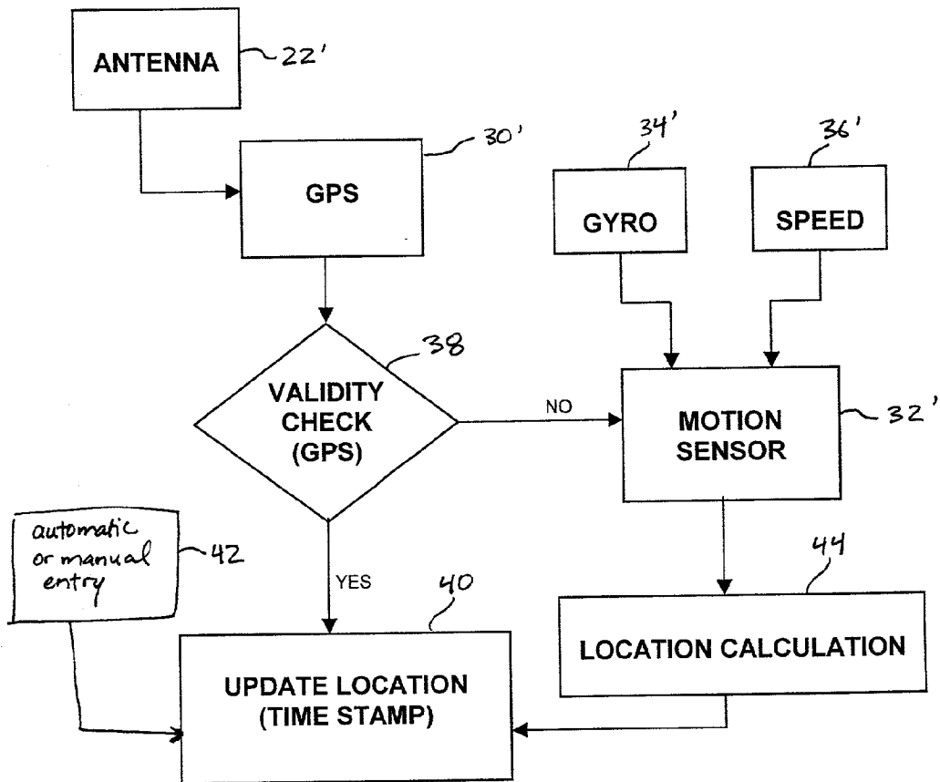
Fig. 3 Data Processing of the Location Module
