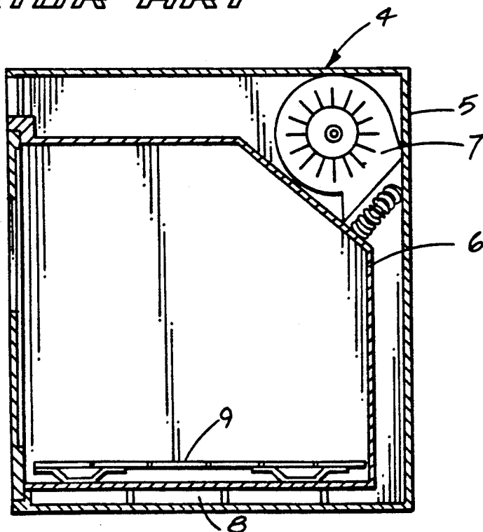
FIG. 2 PRIOR ART
