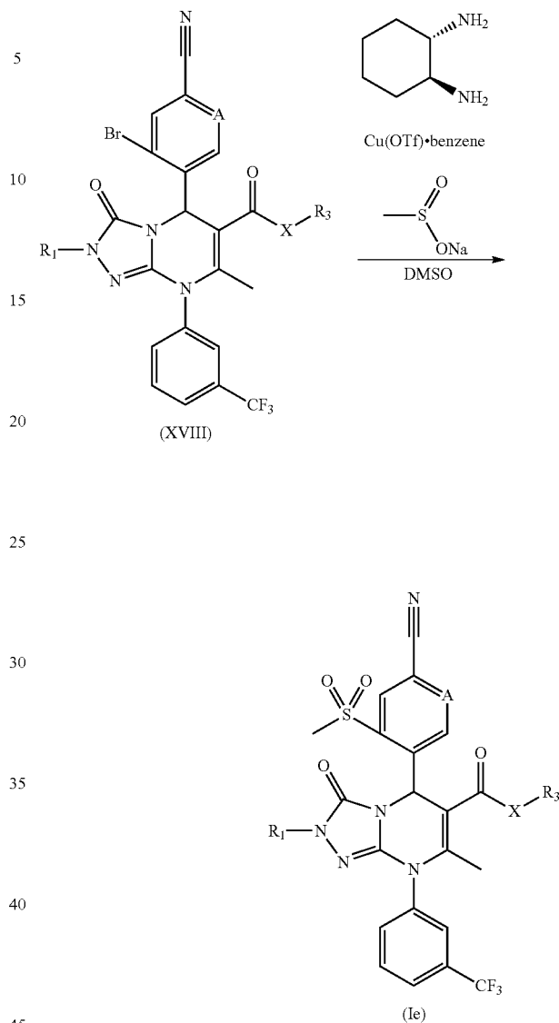
Scheme F:
