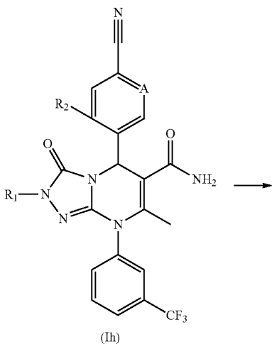
Scheme H:
