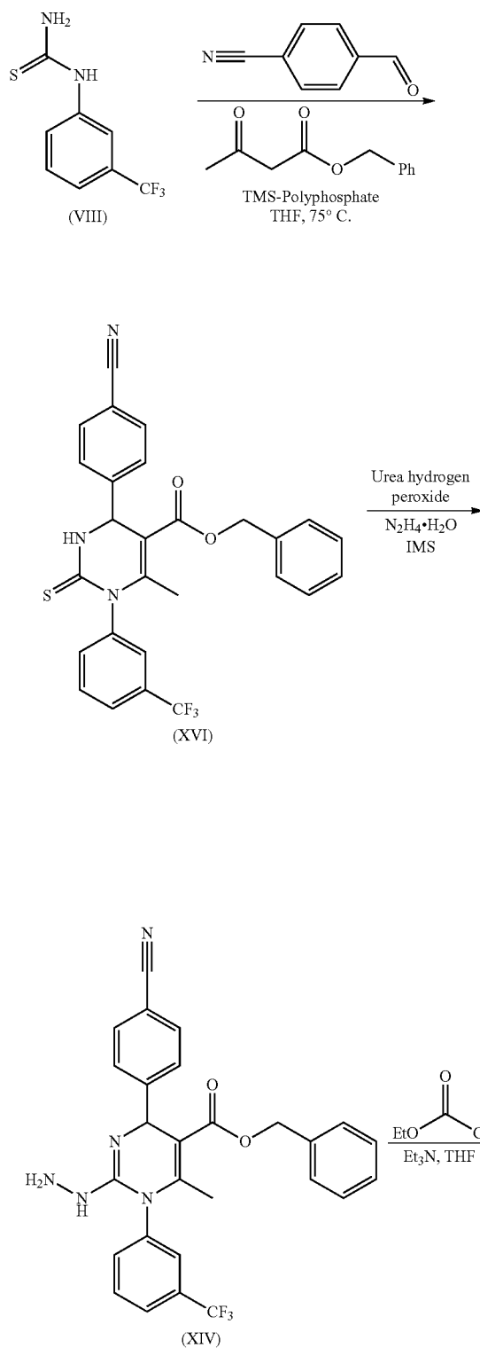
Scheme C:
