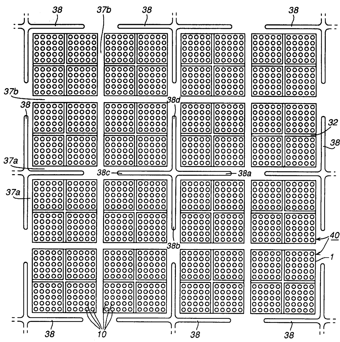
FIG. 4 (PRIOR ART)
