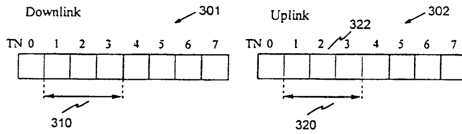
Fig. 3 PRIOR ART
