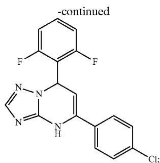
5-(4-chlorophenyl)-7-(2,6-difluorophenyl)-4,7-dihydro[1,2,4]triazolo[1,5-a]pyrimidine
