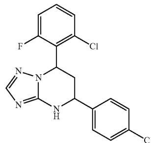
65 7-(2-chloro-6-fluorophenyl)-5-(4-chlorophenyl)-4,5,6,7-tetrahydro[1,2,4]triazolo[1,5-a]pyrimidine
