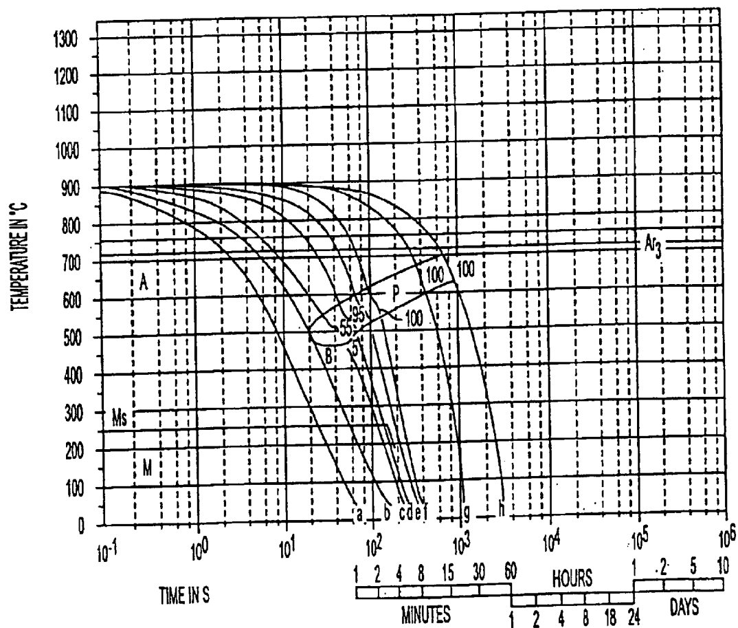
FIG. 3 (PRIOR ART)
