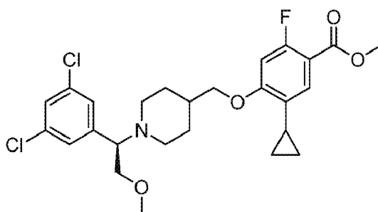
(R)-methyl 5-cyclopropyl-4-((1-(1-(3,5-dichlorophenyl)-2-methoxyethyl)piperidin-4-yl)methoxy)-2-fluorobenzoate
