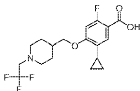
5-Cyclopropyl-2-fluoro-4-((1-(2,2,2-trifluoroethyl)piperidin-4-yl)methoxy)benzoic acid
