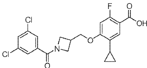
5-Cyclopropyl-4-((1-(3,5-dichlorobenzoyl)azetidin-3-yl)methoxy)-2-fluorobenzoic acid
