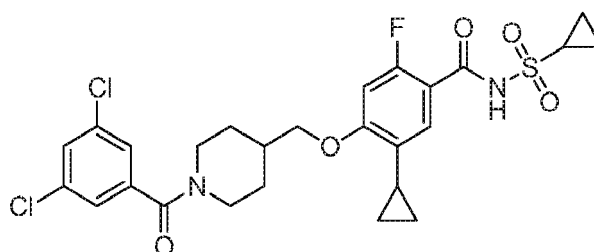
5-Cyclopropyl-N-(cyclopropylsulfonyl)-4-((1-(3,5-dichlorobenzoyl)piperidin-4-yl)methoxy)-2-fluorobenzamide
