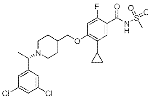
(S)-5-Cyclopropyl-4-((1-(1-(3,5-dichlorophenyl)ethyl)piperidin-4-yl)methoxy)-2-fluoro-N-(methylsulfonyl)benzamide
