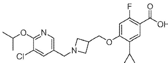
4-((1-((5-Chloro-6-isopropoxypyridin-3-yl)methyl)azetidin-3-yl)methoxy)-5-cyclopropyl-2-fluorobenzoic acid
