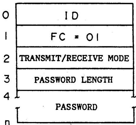
FIG. 4 B (START REQUEST)
