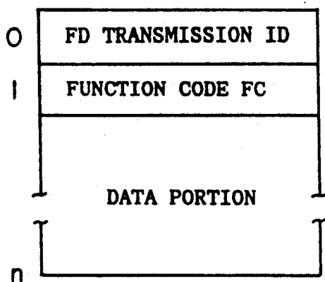
FIG. 4 A (COMMON DATA FORMAT)
