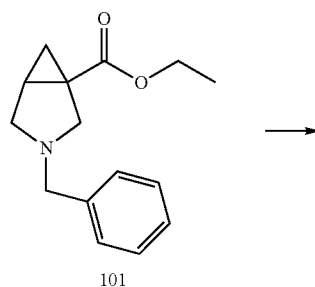
Scheme 101:
