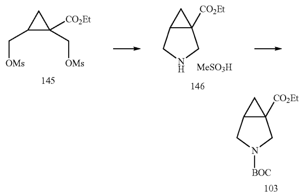
Ethyl 3-azabicyclo[3.1.0]hexane-1-carboxylate (146)
