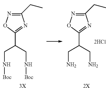
Step 6: 2-(3-ethyl-1,2,4-oxadiazole-5-yl)propane-1,3-diamine dihydrochloride
