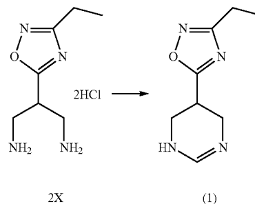
Step 7: 3-ethyl-5-(1,4,5,6-tetrahydropyrimidin-5-yl)-1,2,4-oxadiazole (1):
