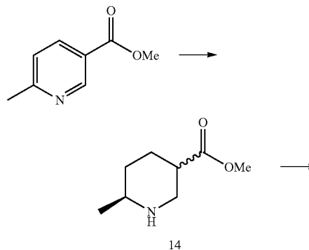
Scheme 12
