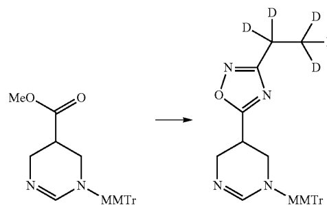
Step 2: 3-(1,1,2,2,2-d 5 -ethyl)-5-(1-((4-methoxyphenyl)diphenylethyl)-1,4,5,6-tetrahydropyrimidine-5-yl)-1,2,4-oxadiazole
