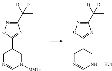
Step 4: 3-(2,2-d 2 -ethyl)-5-(1,4,5,6-tetrahydropyrimidin-5-yl)-1,2,4-oxadiazole hydrochloride
