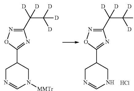
Step 3: 3-(1,1,2,2,2-d 5 -ethyl)-5-(1,4,5,6-tetrahydropyrimidine-5-yl)-1,2,4-oxadiazole hydrochloride
