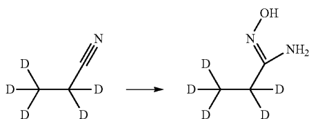
Step 1: 2,3,3,3-d 5 -Propionamideoxime
