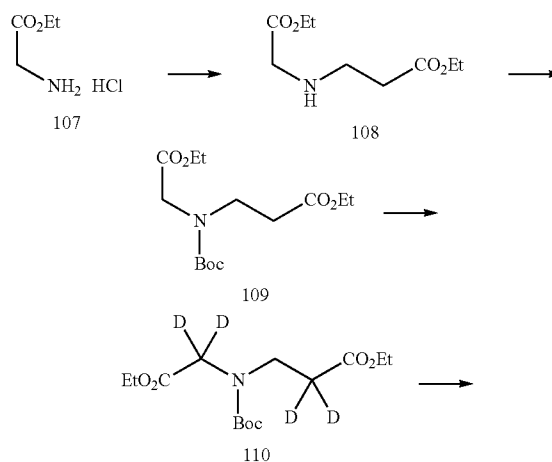
Scheme 102:
