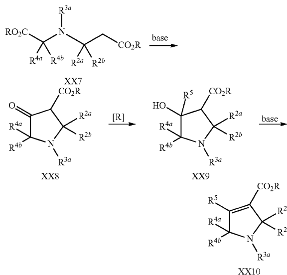
Scheme 11
