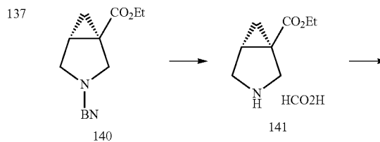
Scheme 104: Enantiospecific synthesis of azabicyclo compounds.
