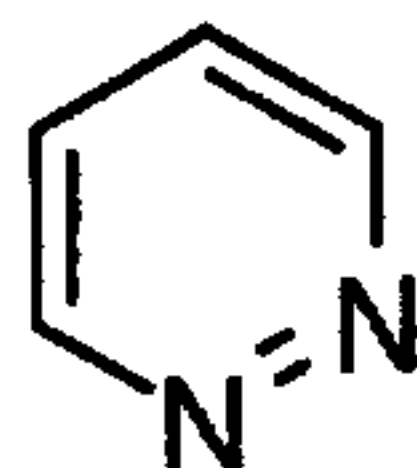
pyridazine (pyridazinyl)
