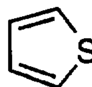
thiophene (thienyl)
