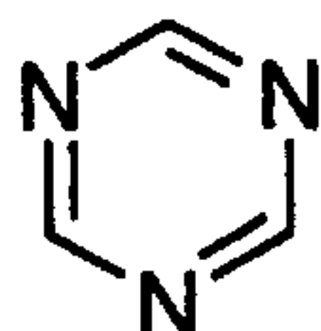
triazine (triazinyl)
