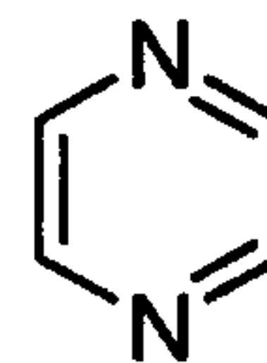
pyrazine (pyrazinyl)
