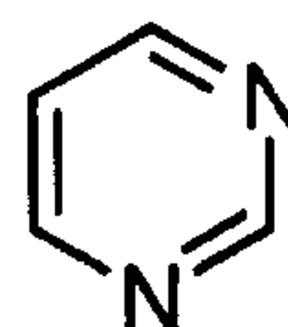
pyrimidine (pyrimidinyl)
