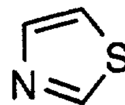
thiazole (thiazolyl)
