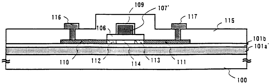
Fig. 2D FORMATION OF INTERLAYER INSULATING FILM 115 AND WIRE
