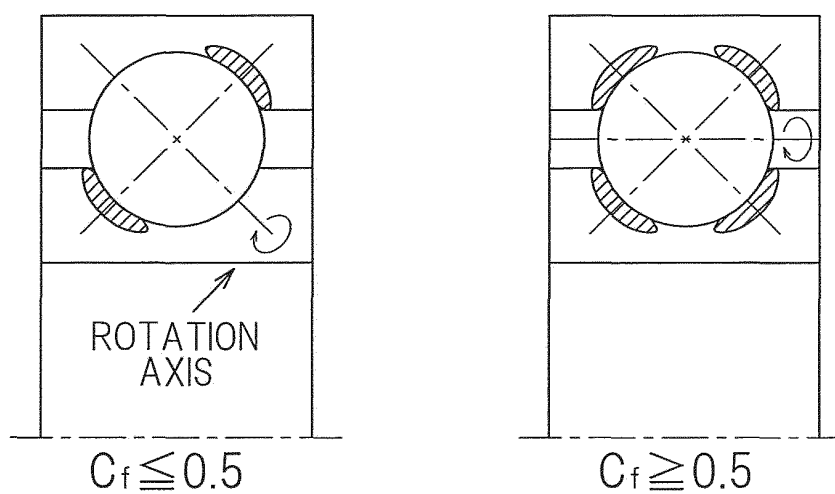
RELATION OF C_f AND ROTATION AXIS
