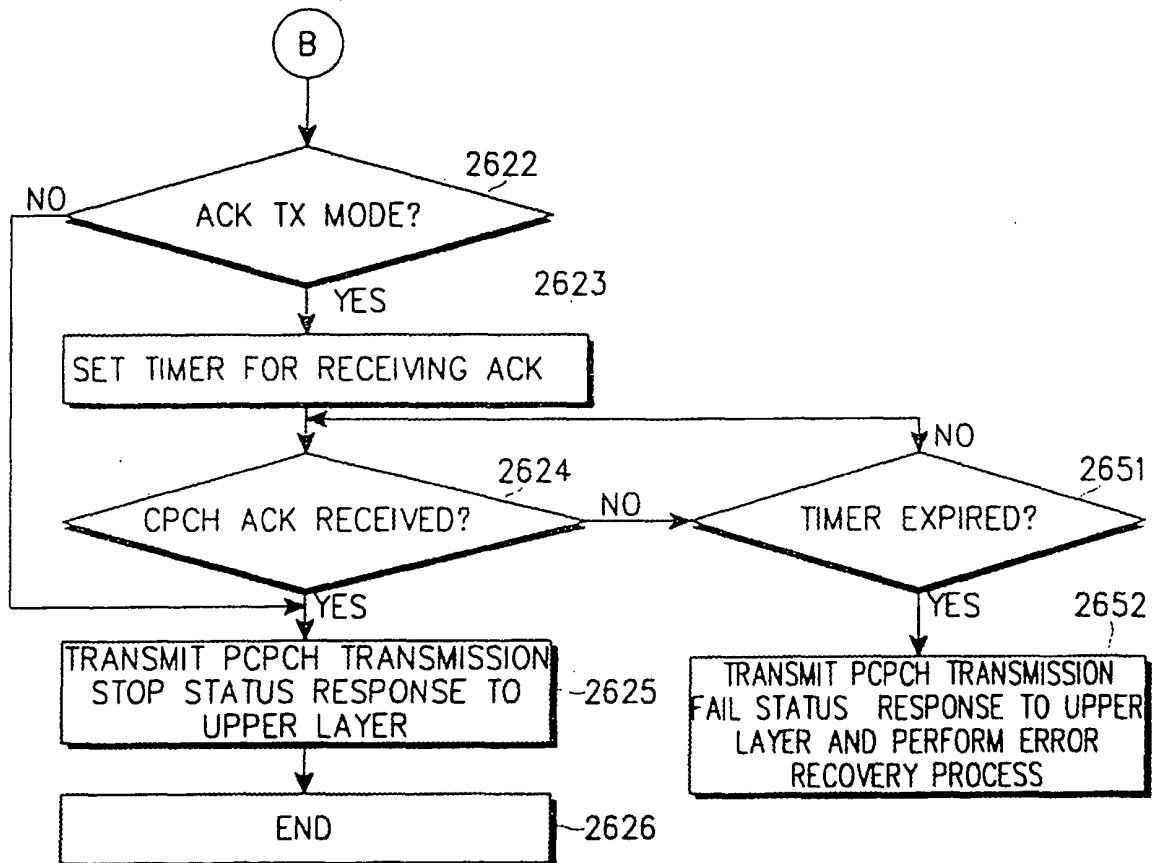
FLOWCHART OF CPCH USING CHANNEL ASSIGNMENT (UE SIDE)
