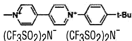
1-methyl-1'-(4-tert-butylphenyl)-4,4'- bipyridinium bis(trifluoromethanesulfonylimide) (21)
