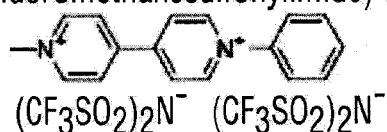
1-methyl-1'-phenyl-4,4'-bipyridinium bis(trifluoromethanesulfonylimide) (19)
