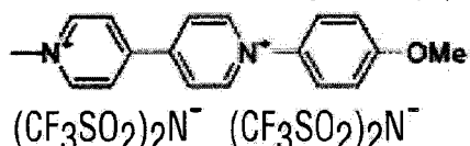
1-methyl-1'-(4-trifluoromethylphenyl)-4,4'- bipyridinium bis(trifluoromethanesulfonylimide) (23)
