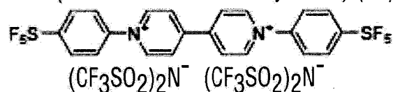
1,1'-bis(4-(pentafluoro-λ 6 -sulfanyl)phenyl)- 4,4'-bipyridinium bis(trifluoromethanesulfonylimide) (17)
