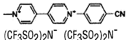
1-methyl-1'-(4-cyanophenyl)-4,4'- bipyridinium bis(trifluoromethanesulfonylimide) (24)
