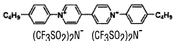
1,1'-bis(4-butylphenyl)-4,4'-bipyridinium bis(trifluoromethanesulfonylimide) (13)
