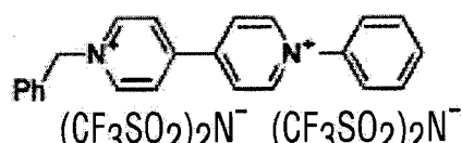
1-benzyl-1'-phenyl-4,4'-bipyridinium bis(trifluoromethanesulfonylimide) (20)
