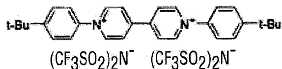
1,1'-bis(4-tert-butylphenyl)-4,4'-bipyridinium bis(trifluoromethanesulfonylimide) (14)
