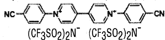
1,1'-bis(4-cyanophenyl)-4,4'-bipyridinium bis(trifluoromethanesulfonylimide) (18)
