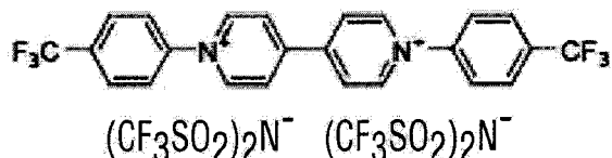
1,1'-bis(4-trifluoromethylphenyl)-4,4'- bipyridinium bis(trifluoromethanesulfonylimide) (15)
