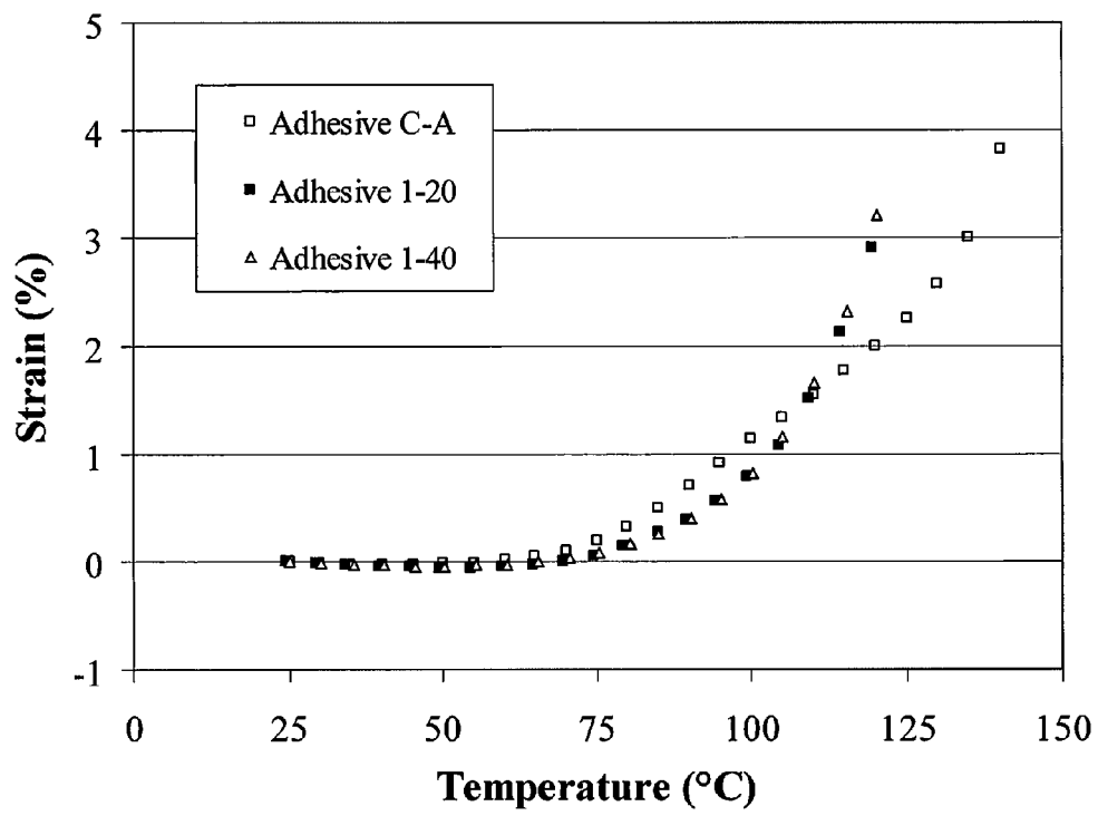
Strain vs. Temperature
