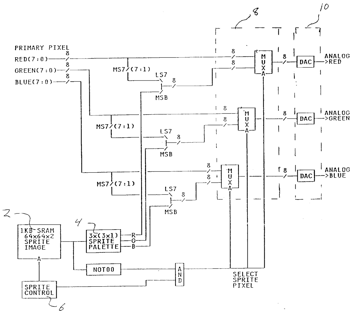
FIGURE - Semi-Translucent Sprite/Cursor Circuitry
