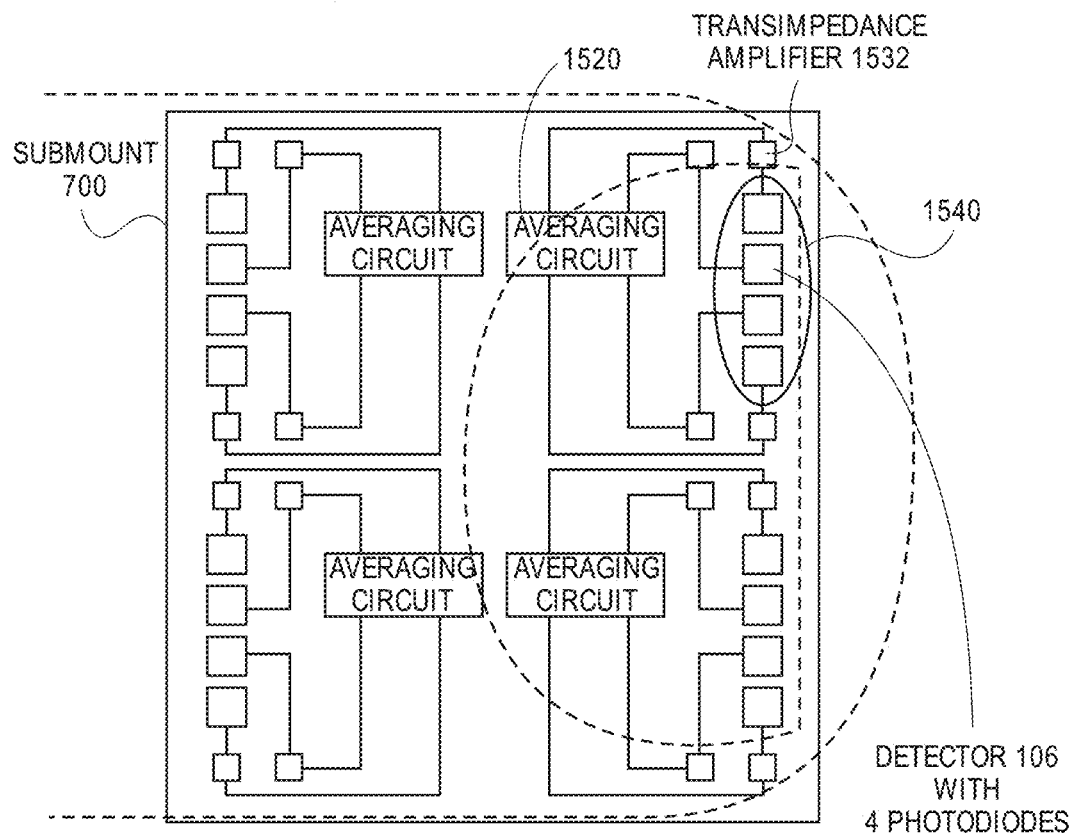
1 PD PER STREAM ARCHITECTURE
