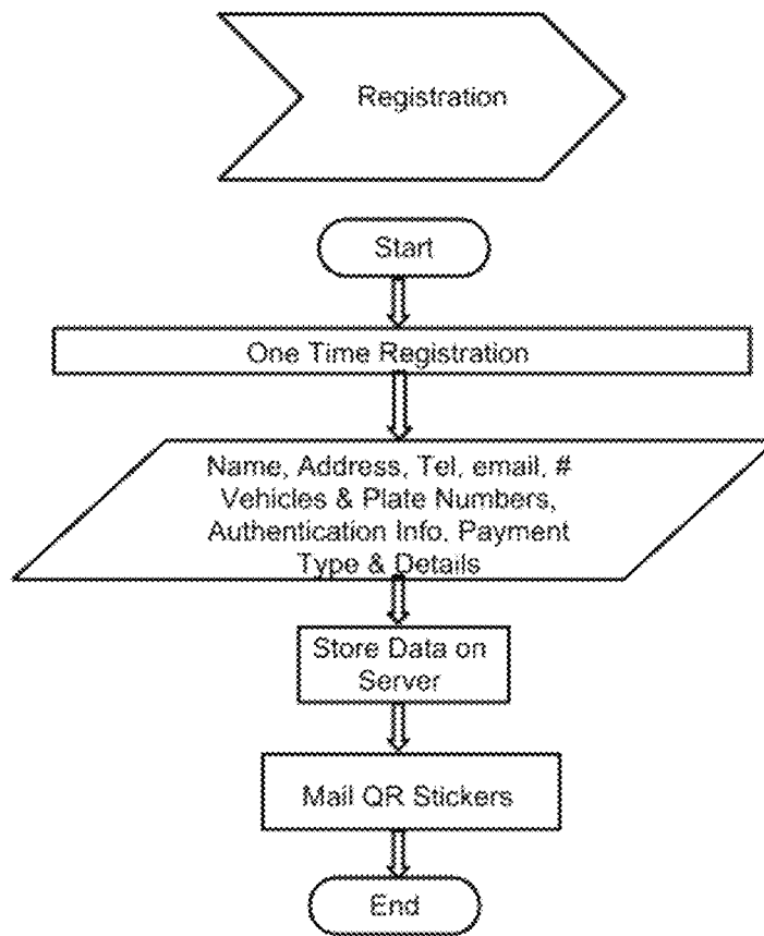
Fig 4 Flow Chart for Registration
