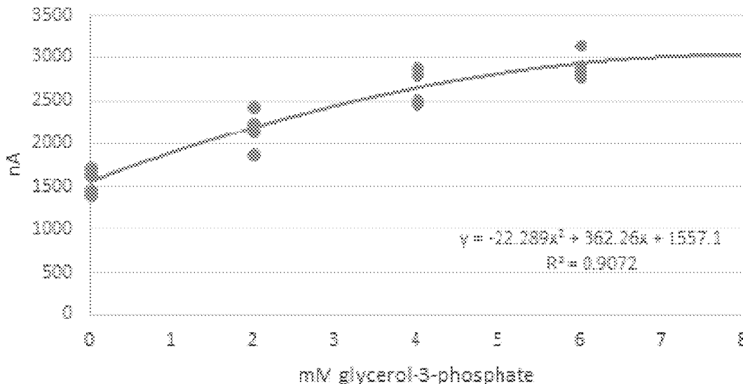
E-glycerol-3-phosphate at 10 Seconds (400 mV)
