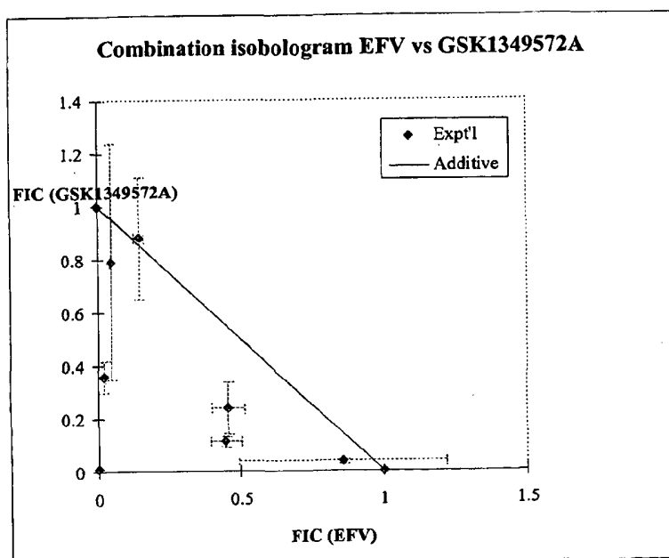
Figure 2: Inhibition of HIV-1 IIIB by a compound of formula (I), GSK1349572A, in combination with efavirenz (EFV).
