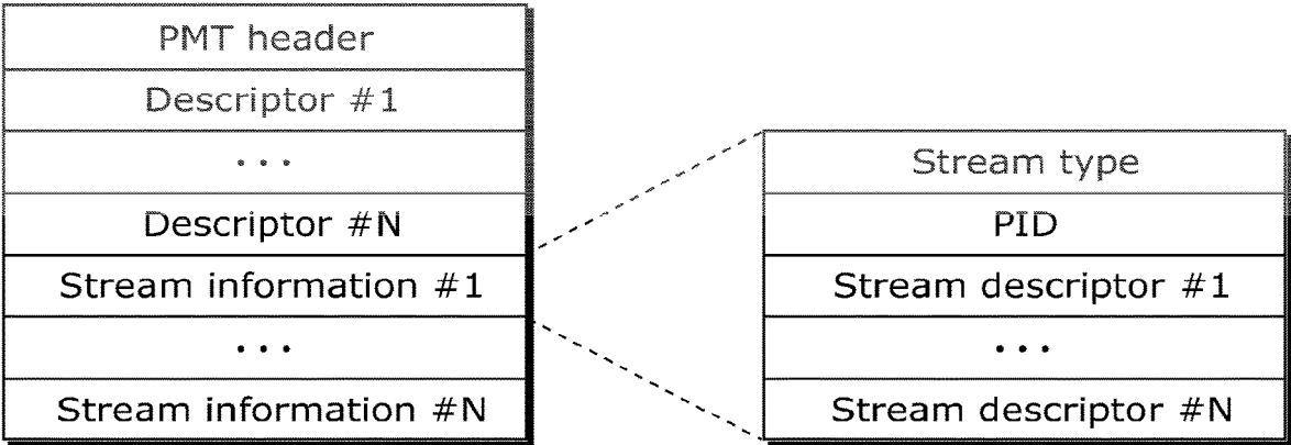
Data structure of PMT
