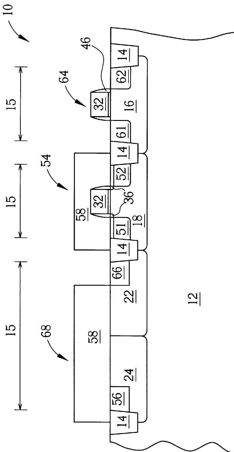
Fig. 6 Prior art
