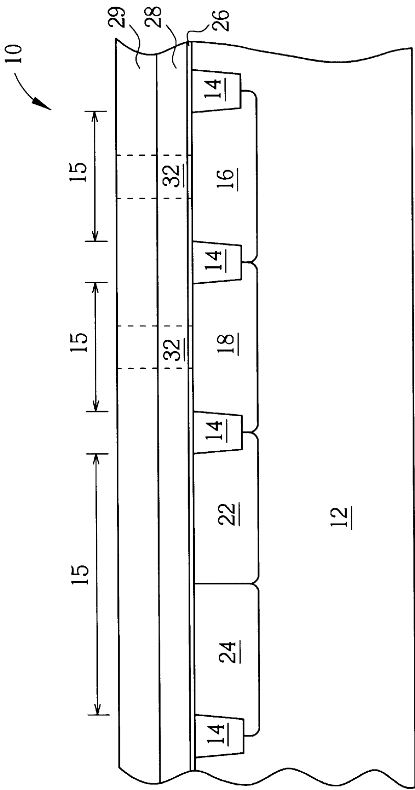
Fig. 2 Prior art
