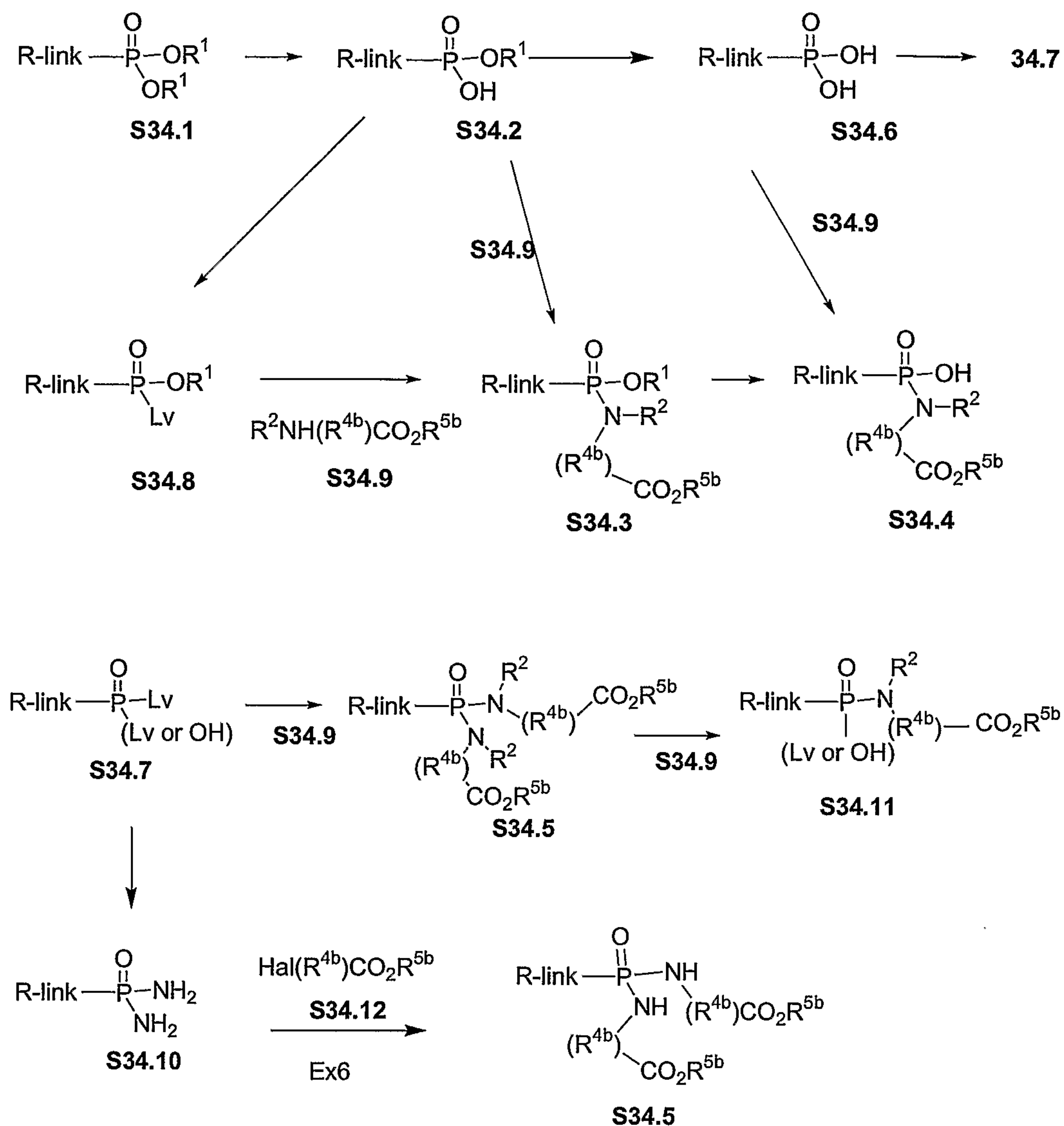
Scheme 34
