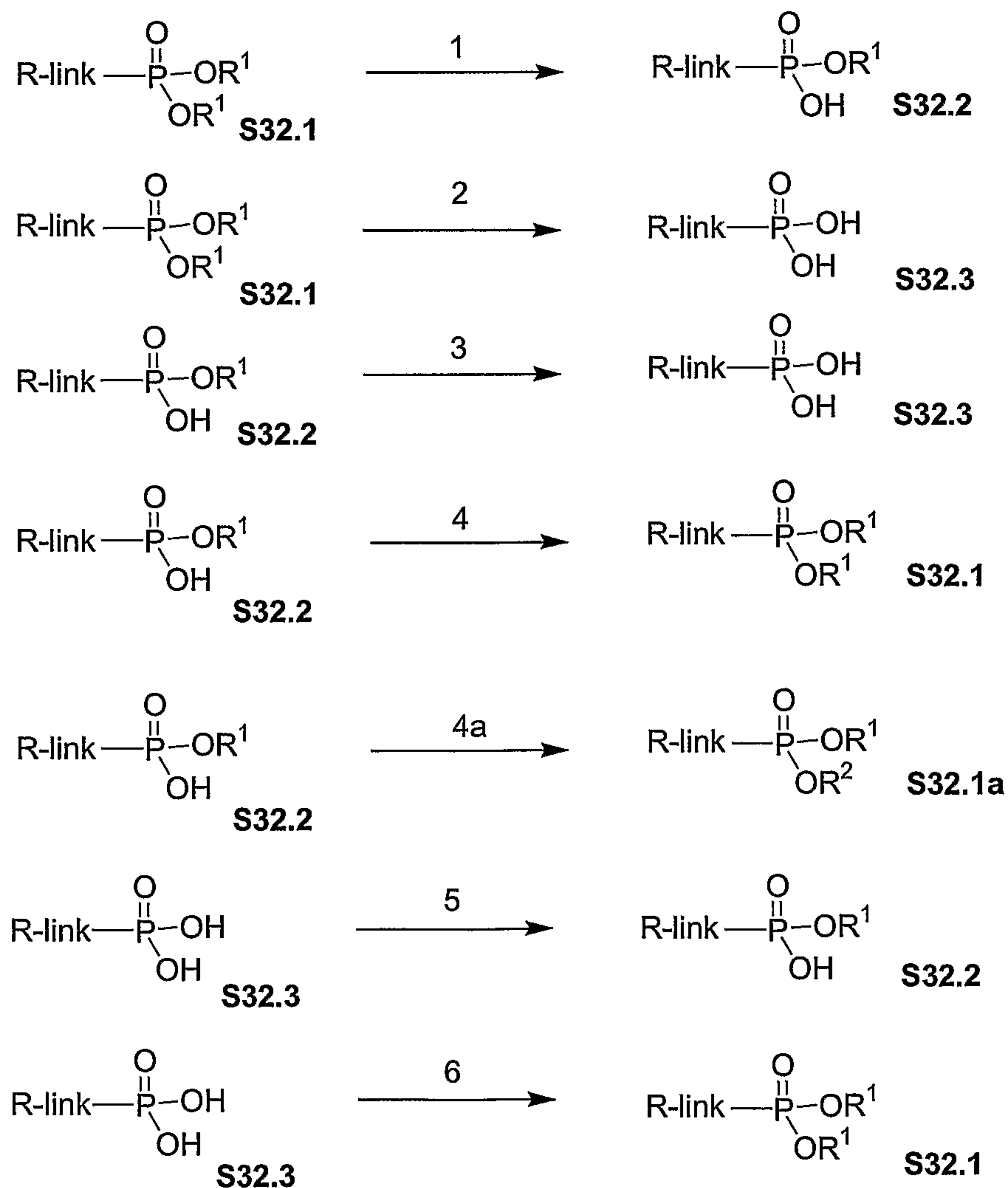
Scheme 32
