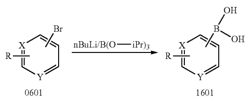
Scheme 16
