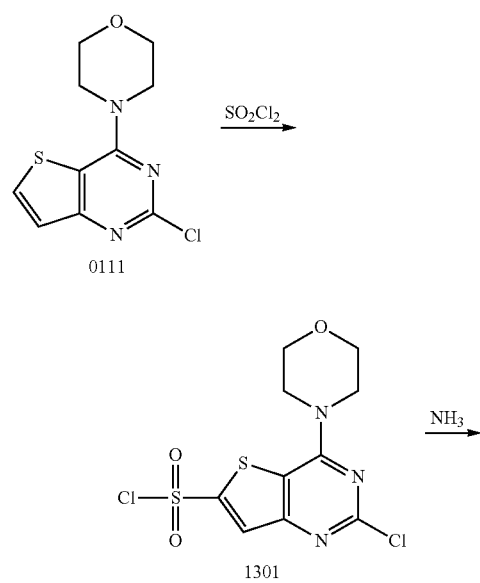
Scheme 13
