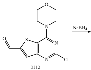
Scheme 5
