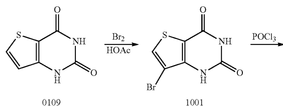
Scheme 10
