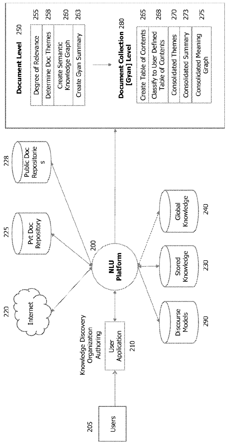
Fig. 2 The NLU Platform High Level Architecture
