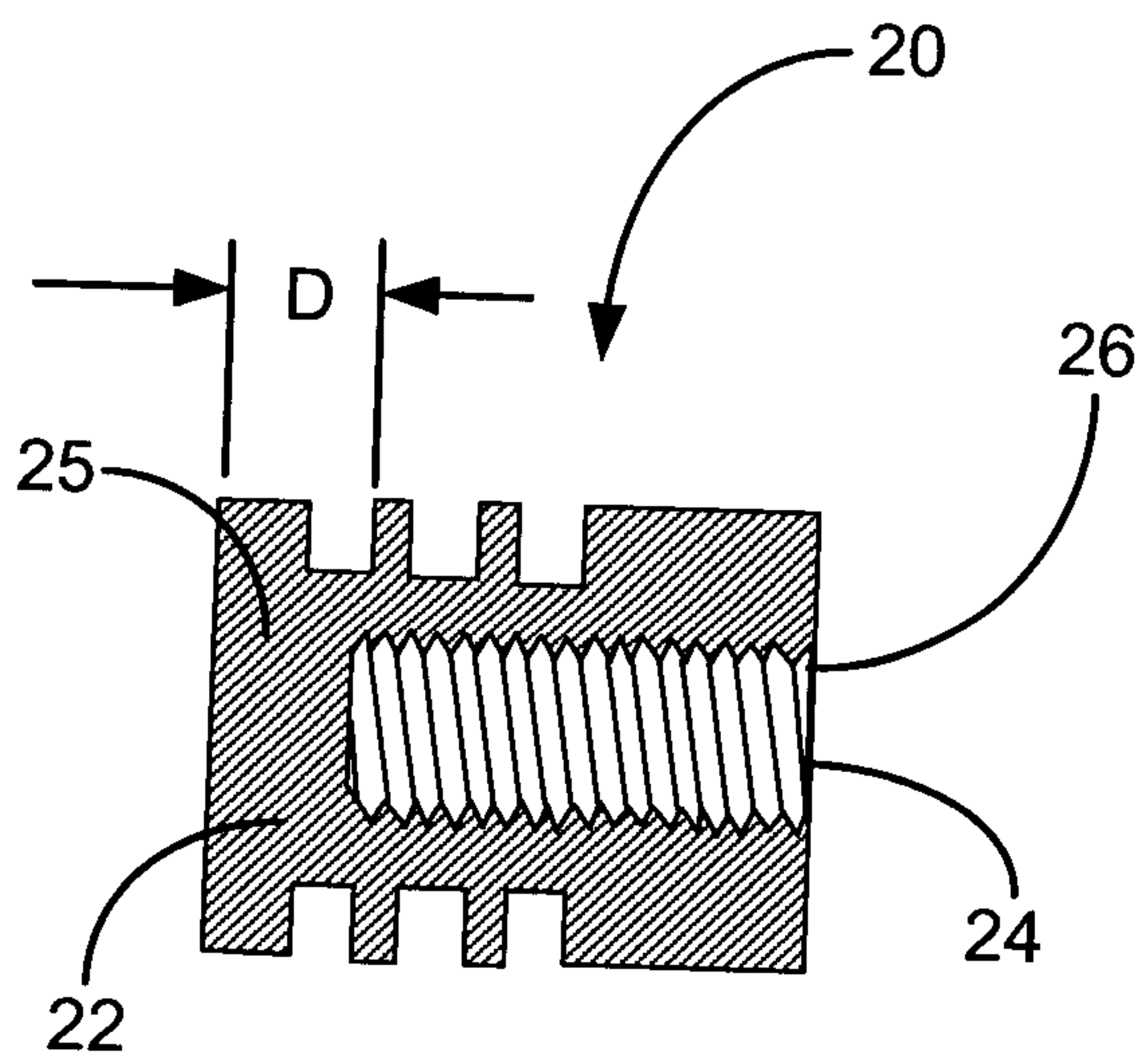
SECTION E-E FIG. 14
