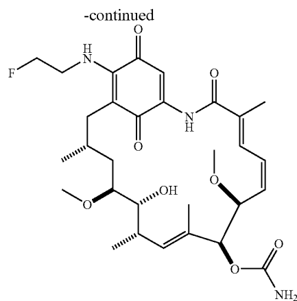
17-fluoroethylaminogeldanamycin
