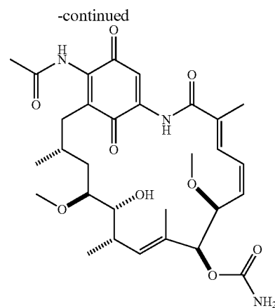
17-acetylgeldanamycin
