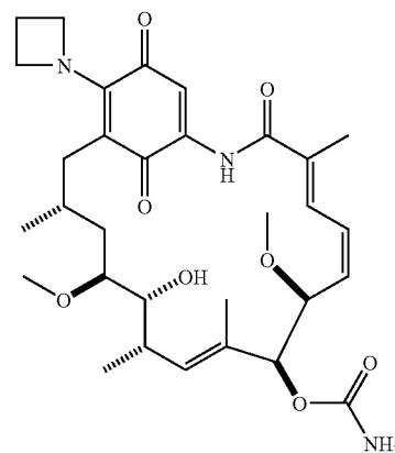
17-azetidinylgeldanamycin
