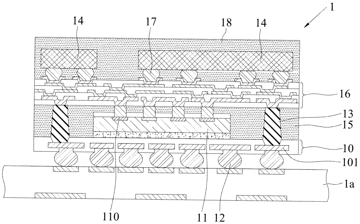
FIG. 1-1 (PRIOR ART)
