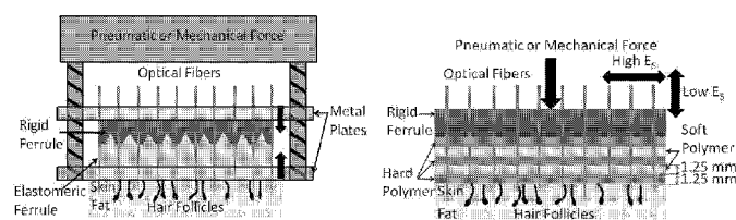
Fiberoptic Microneedle Device (FMD) Schematic Illustration of: (left) device using compression between two rigid plates, and (right) device using layered elastomeric ferrule
