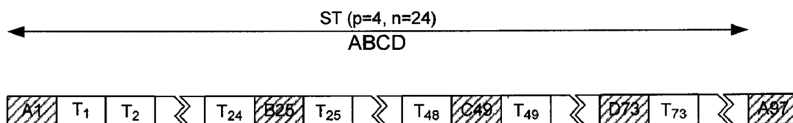
FIG. 9 (PRIOR ART)
