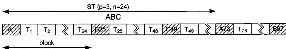
FIG. 7 (PRIOR ART)
