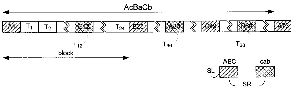
FIG. 9 (PRIOR ART)
