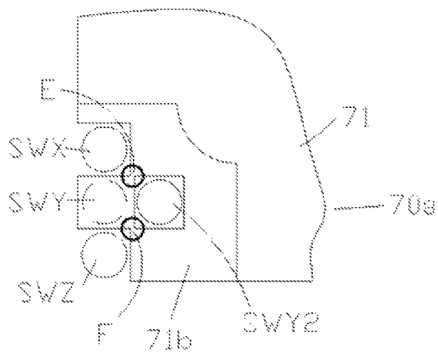
FIG. 29 (PRIOR ART)
