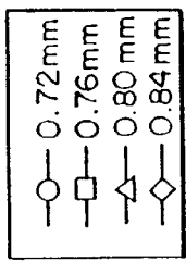
SUBSTRATE THICKNESS FOR NO SPHERICAL ABERRATION IN THE INNER REGION OF THE LENS
