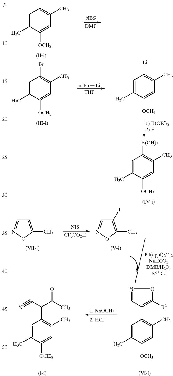
Scheme 9
