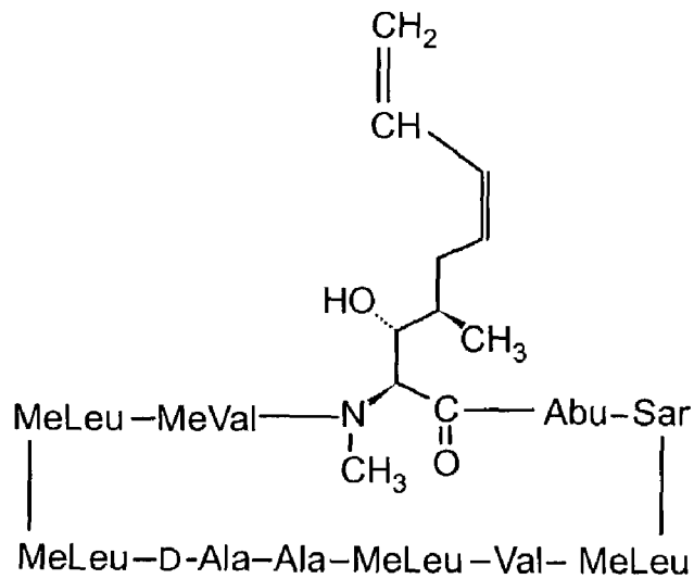
Z-isomer of ISA tx 247
