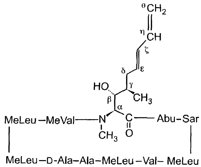
E-isomer of ISA tx 247
