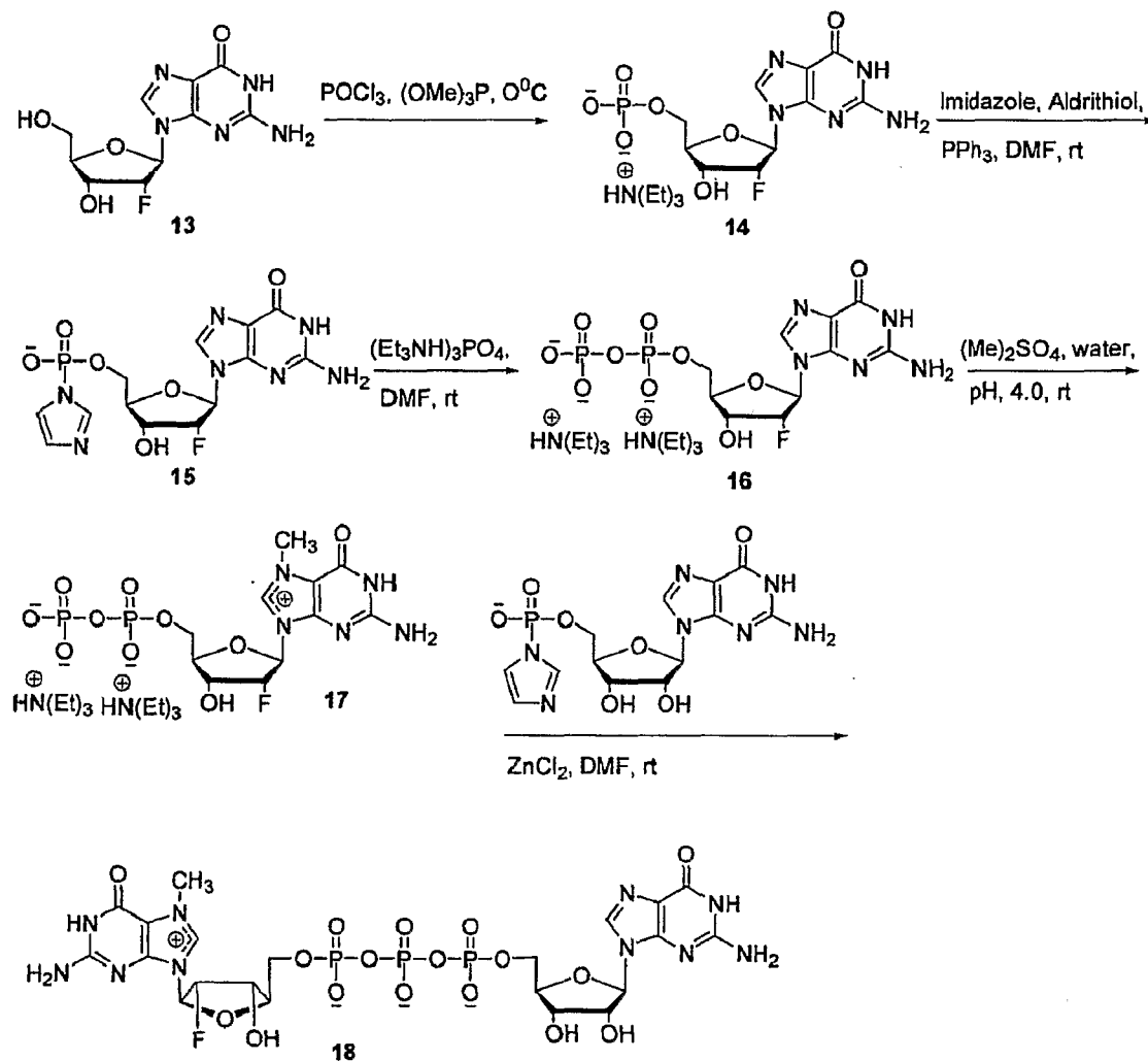
Figure 2: Synthesis of Novel Cap Analog m 7,2'F G[5]ppp[5']G (2'F-Me-7-G(5')ppp(5')G)
