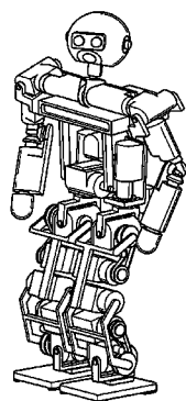
1 LEGGED MOVING ROBOT (FRONT)
