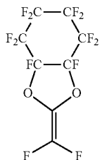
Perfluoro-3-methylene-2,4-dioxabicyclo-[4,3,0]nonane (Monomer E)
