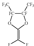
Perfluoro-2-methylene-4,5-dimethyl-1,3-dioxolane (Monomer D)
