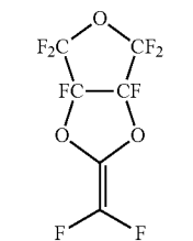
Perfluorotetrahydro-2-methylene-furo[3,4-d][1,3]-dioxolane (Monomer A)
